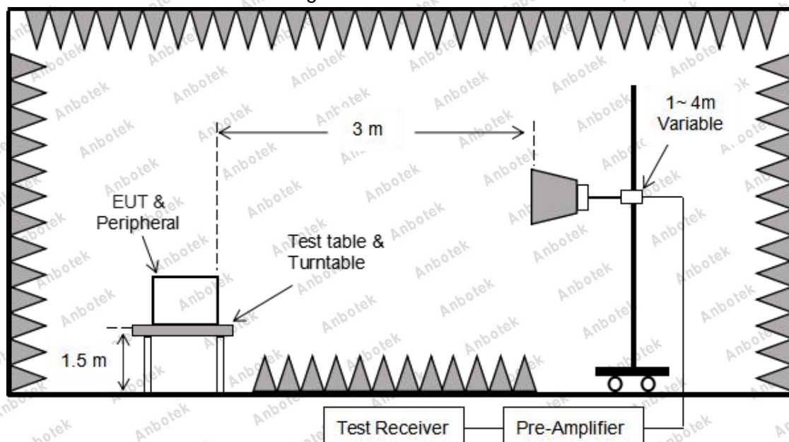
Figure 3. Above 1 GHz
