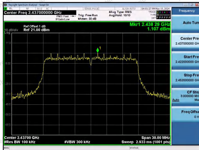
11N20SISO-Ant1-2437-0~Reference-PASS
