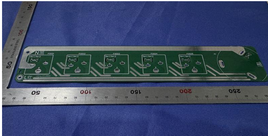
(AC output receptacle board_6pcs)
