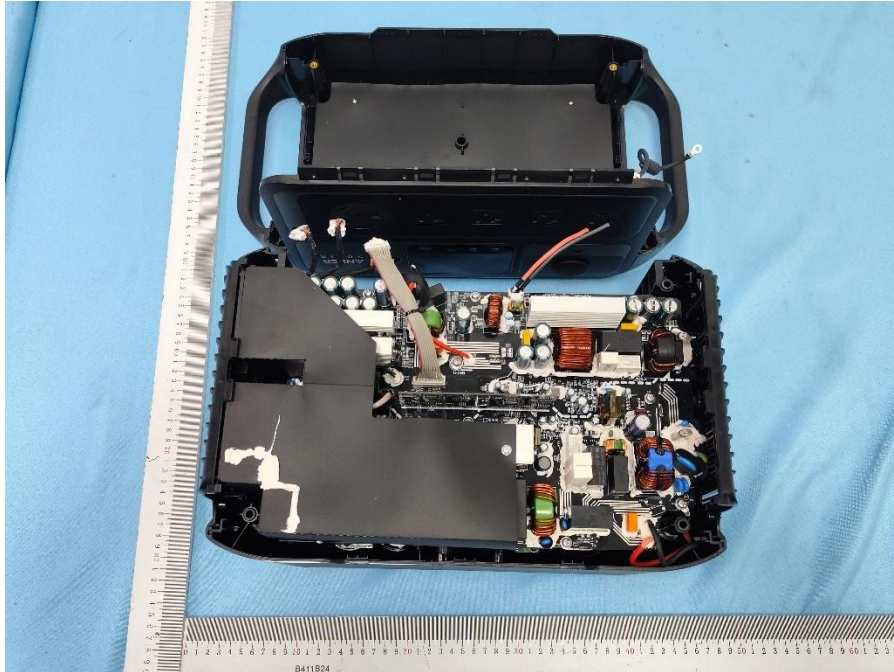
Internal photos of A1785:
