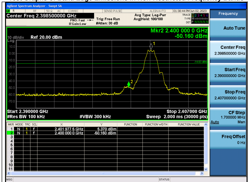
Test Graph LE1M ANT1 2402 1Mbps Lower Band Edge Emissions
