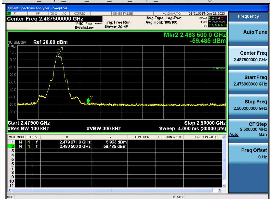
Test Graph LE1M ANT1 2480 1Mbps Higher Band Edge Emissions
