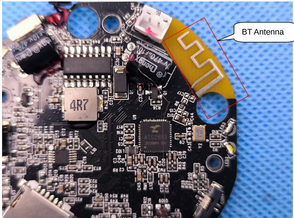
ANTENNA CLOSE-UP PHOTO-1
