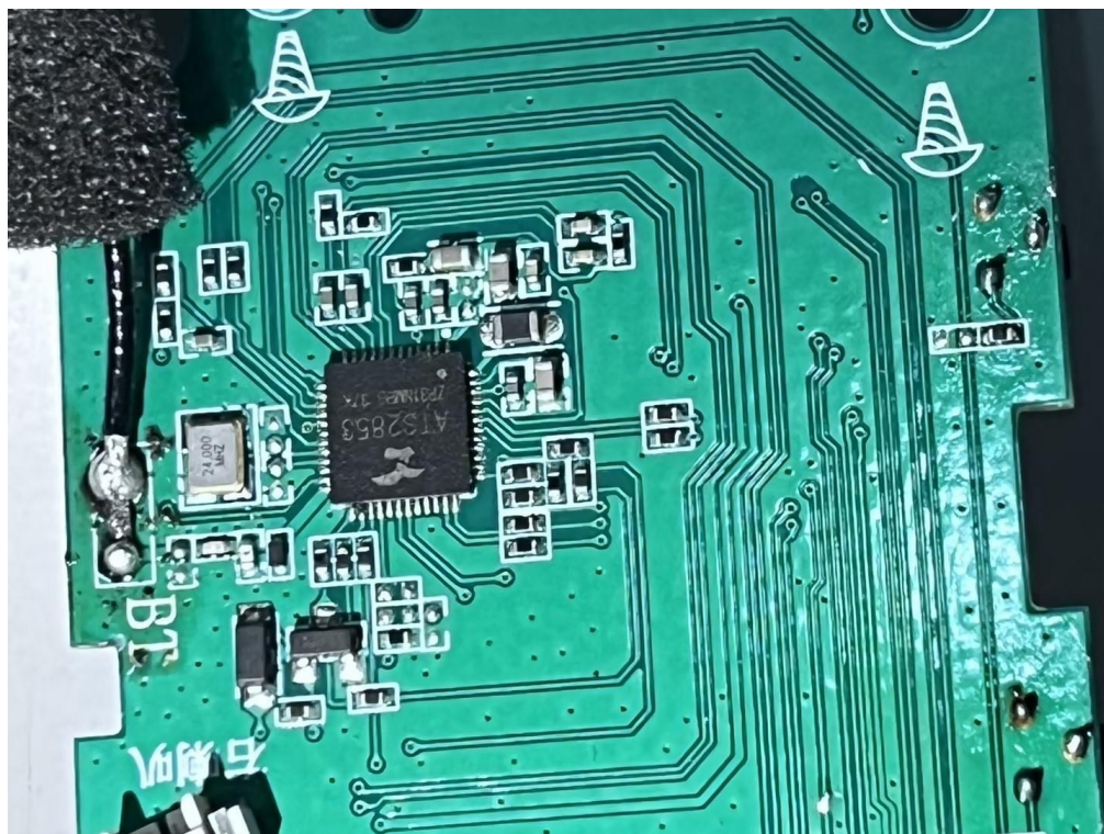
INTERNAL VIEW OF EUT (FIGURE 3) - Updated
