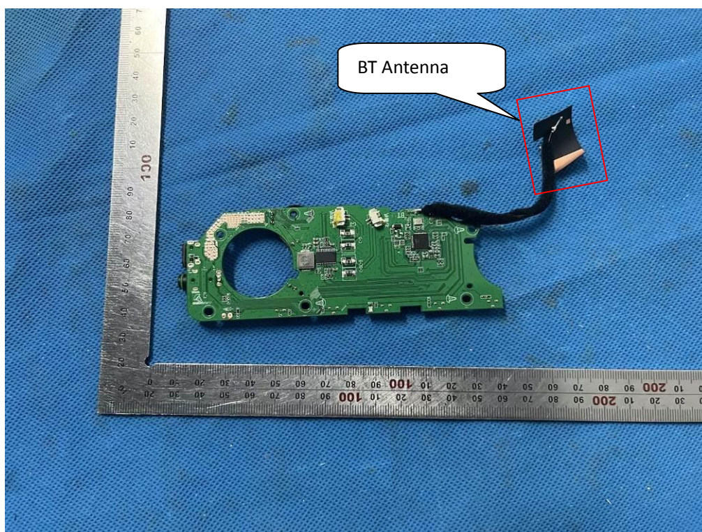
INTERNAL VIEW OF EUT (FIGURE 2) - Updated
