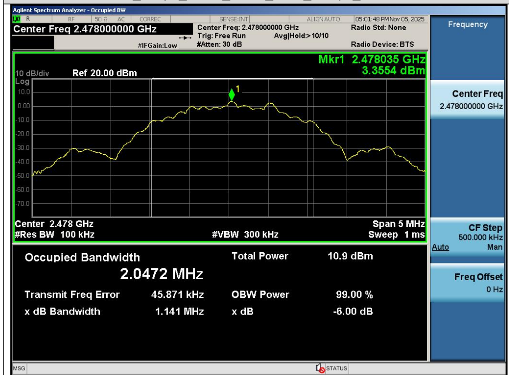
Test_Graph_LE2M_ANT1_2478_2Mbps_DTSBW
