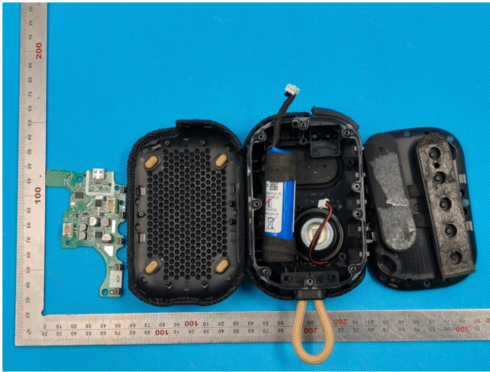
INTERNAL VIEW OF EUT (FIGURE 1)-without spring plate
