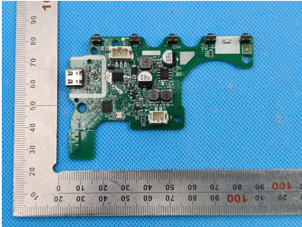
INTERNAL VIEW OF EUT (FIGURE 5) -with spring plate
