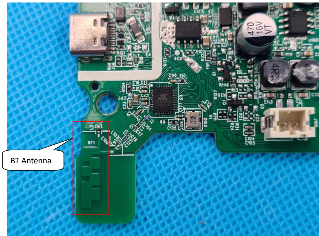
INTERNAL VIEW OF EUT (FIGURE 3) -without spring plate
