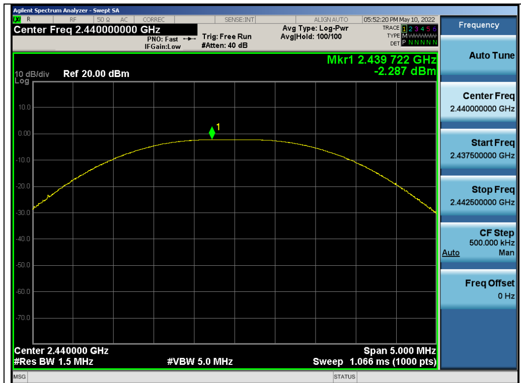
Test_Graph_2.4G_ANT1_2440_Peak Power
