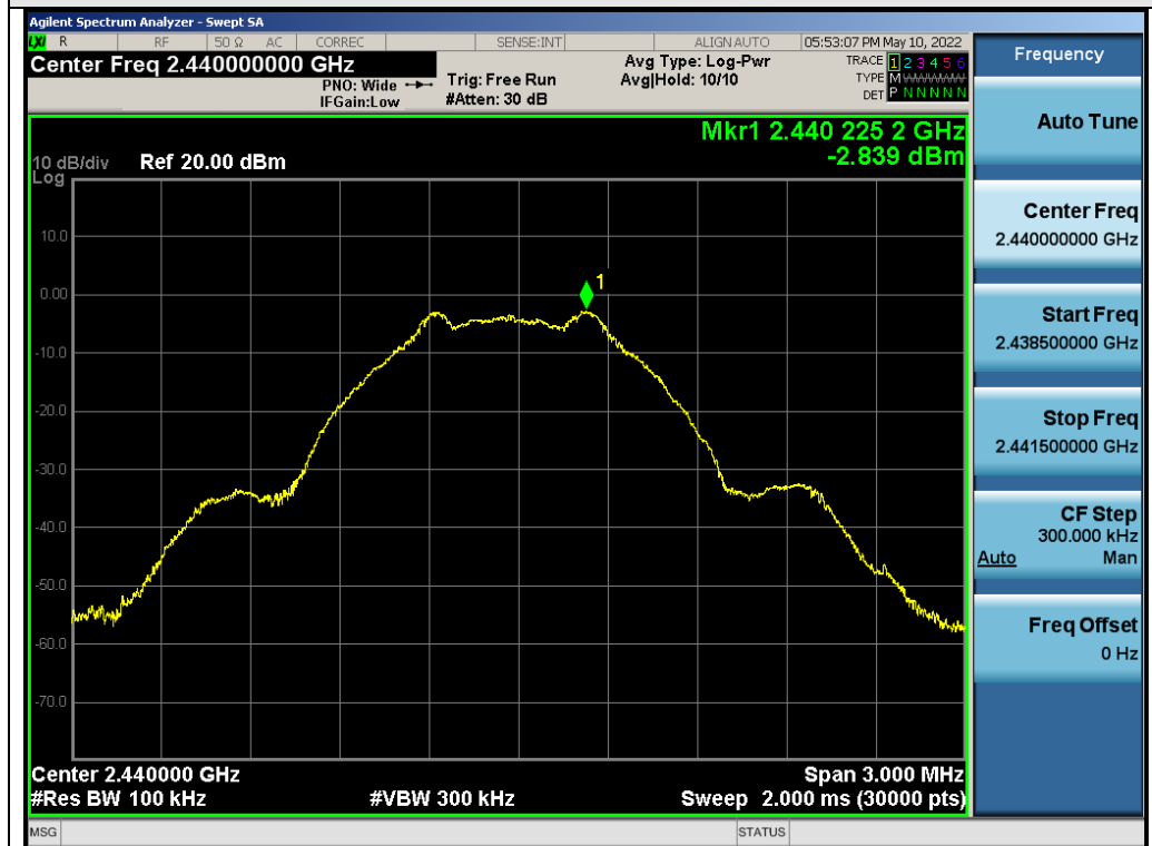
Test_Graph_2.4G_ANT1_2440_Reference Level
