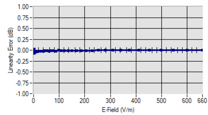
Linearity
