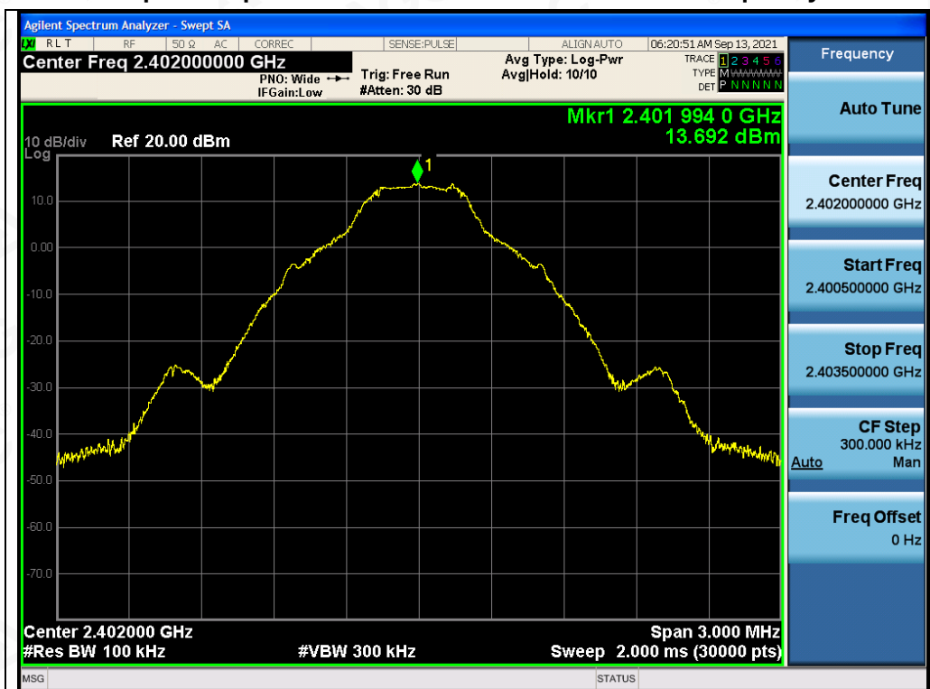
Test Graph BR ANT1 2402 1Mbps Reference Level
