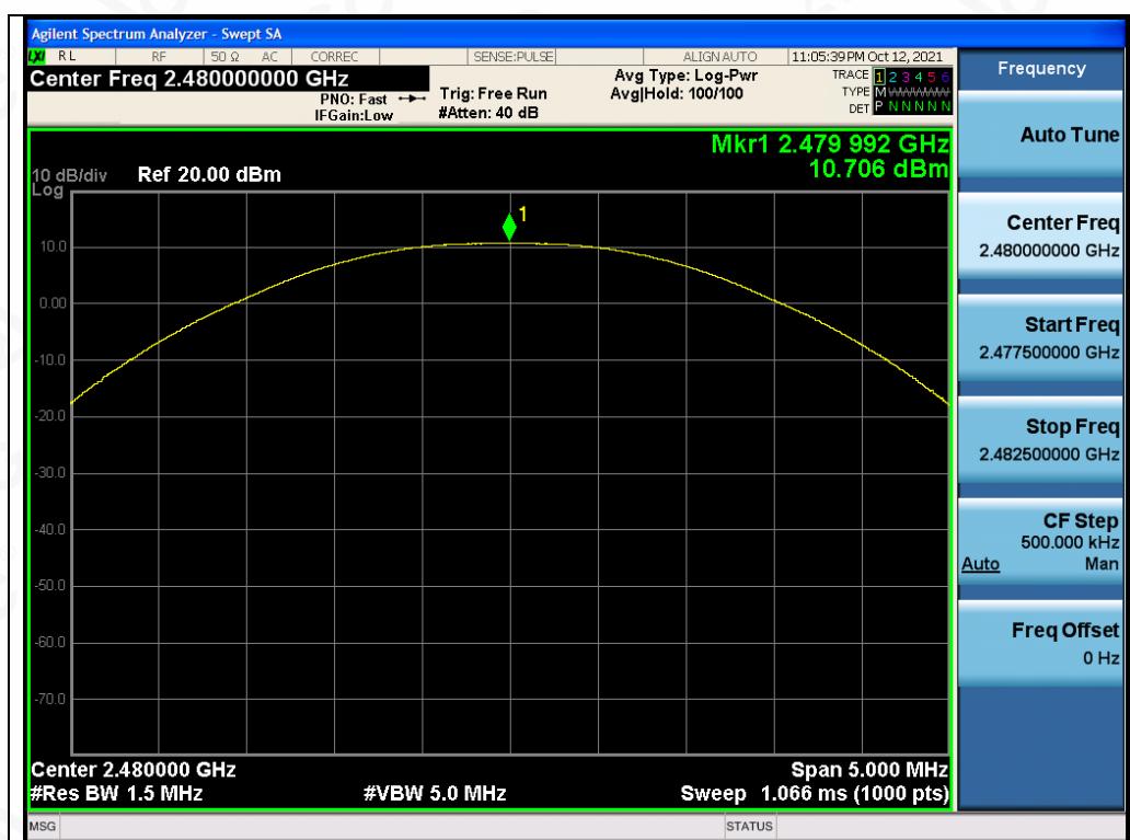
Test Graph EDR ANT1 2480 2Mbps Peak Power
