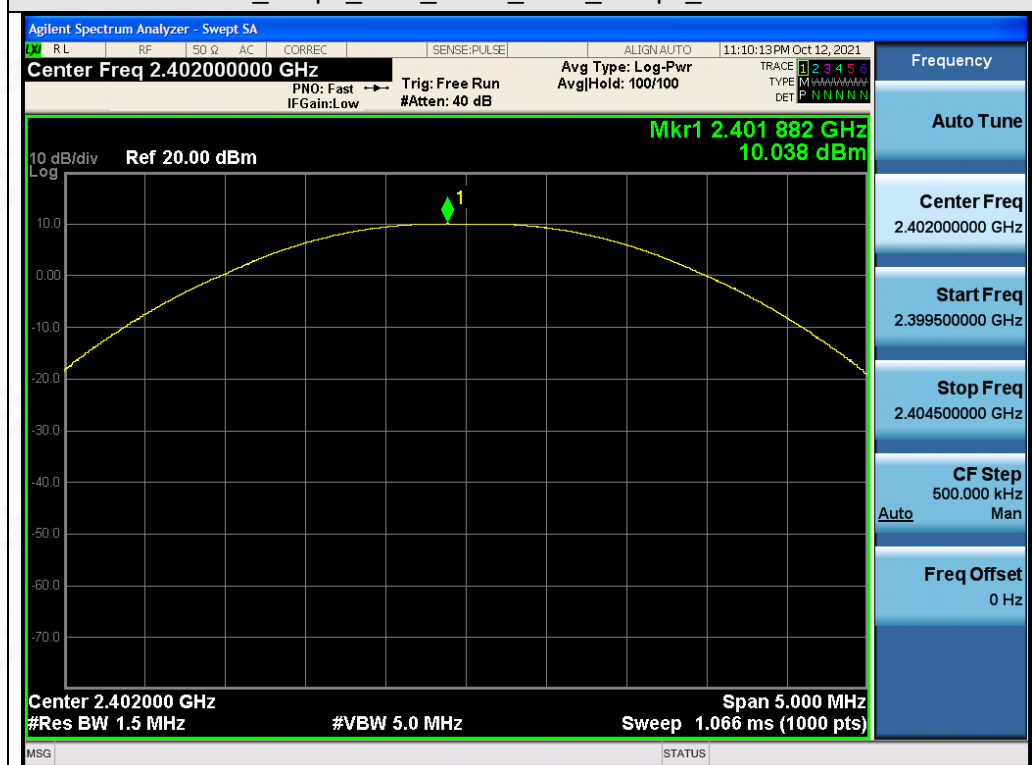
Test Graph EDR ANT1 2402 3Mbps Peak Power
