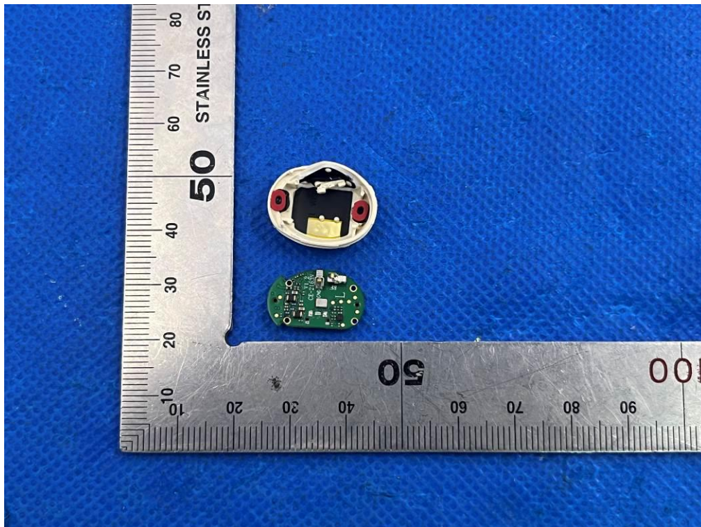
OPEN VIEW OF EUT (FIGURE 1) -Beige white color
