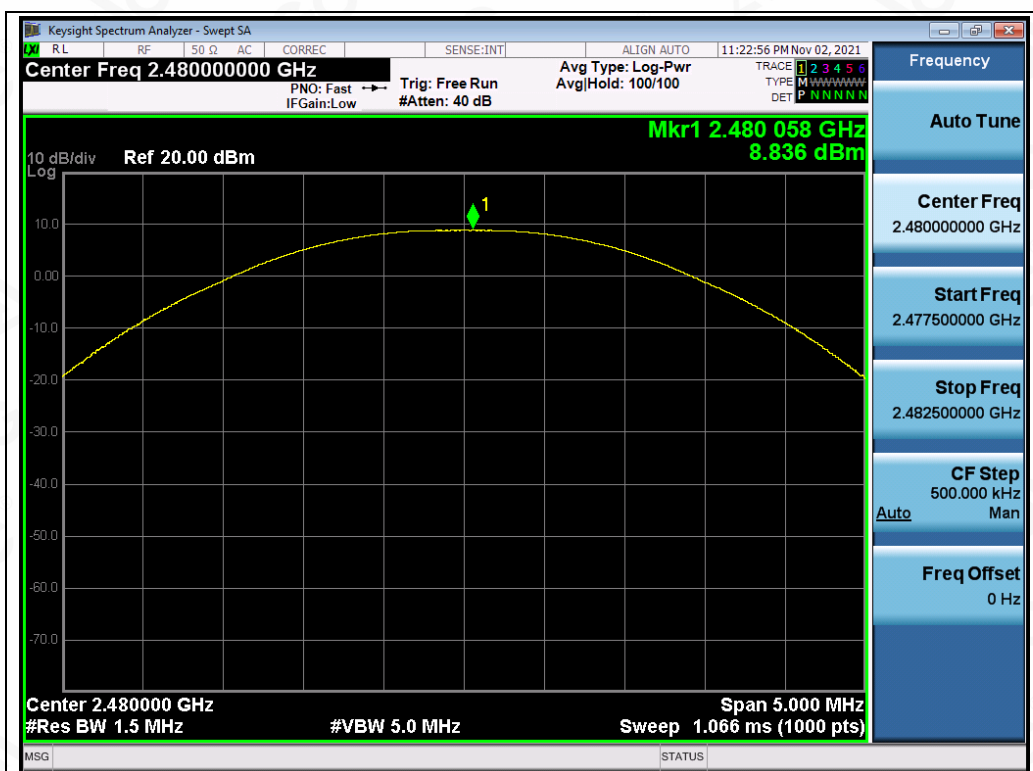
Test_Graph_EDR_ANT1_2480_2Mbps_Peak Power
