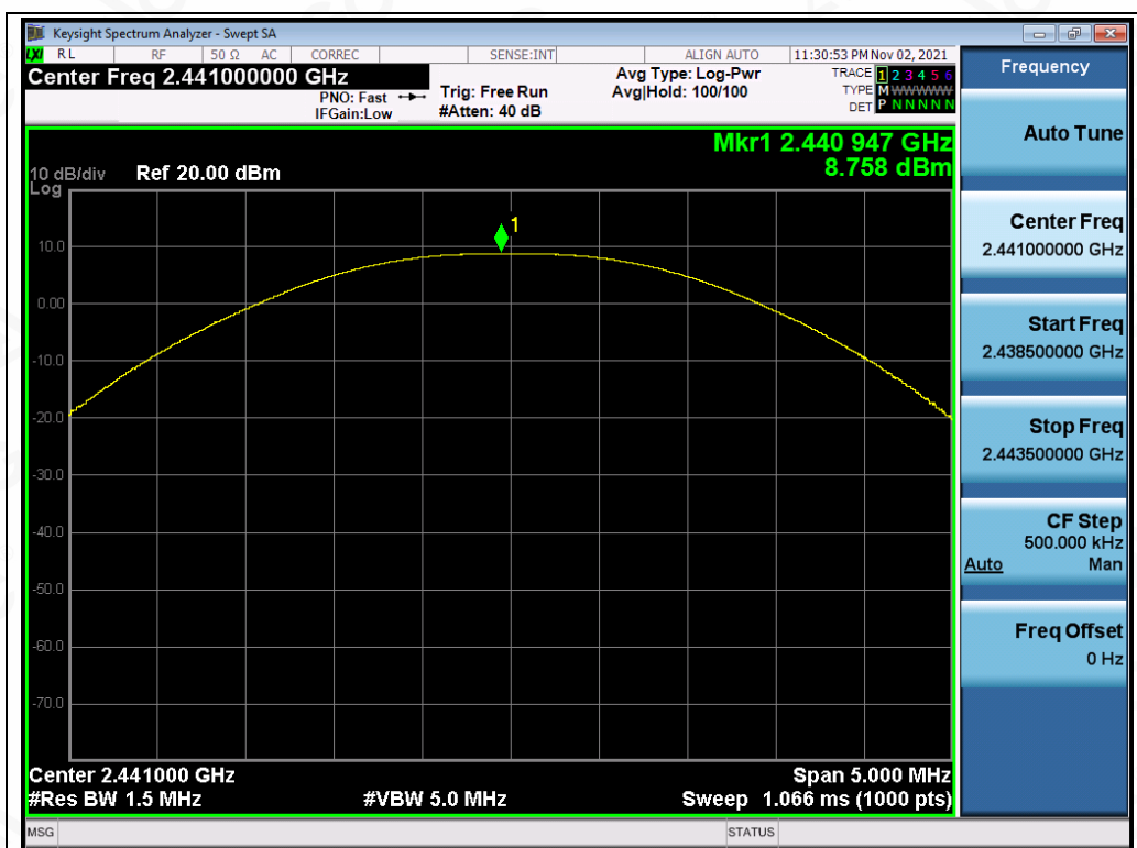
Test_Graph_EDR_ANT1_2441_3Mbps_Peak Power
