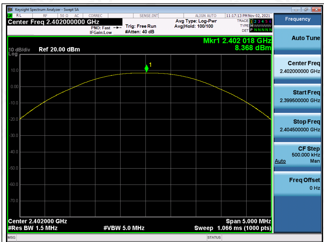
Test_Graph_EDR_ANT1_2402_2Mbps_Peak Power
