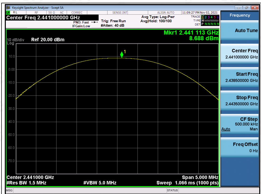
Test_Graph_BR_ANT1_2441_1Mbps_Peak Power
