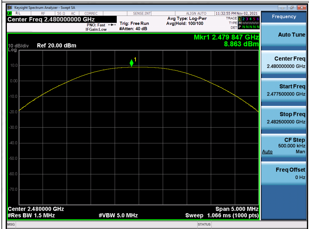
Test_Graph_EDR_ANT1_2480_3Mbps_Peak Power
