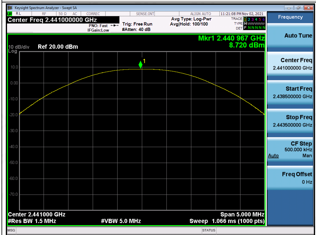
Test_Graph_EDR_ANT1_2441_2Mbps_Peak Power
