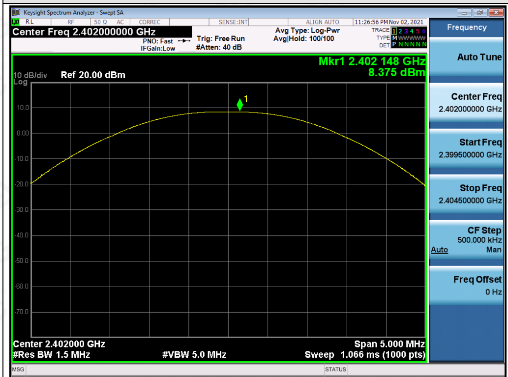
Test_Graph_EDR_ANT1_2402_3Mbps_Peak Power
