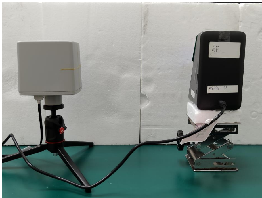
Photograph 9: Set-up for H-field strength (Right View)
