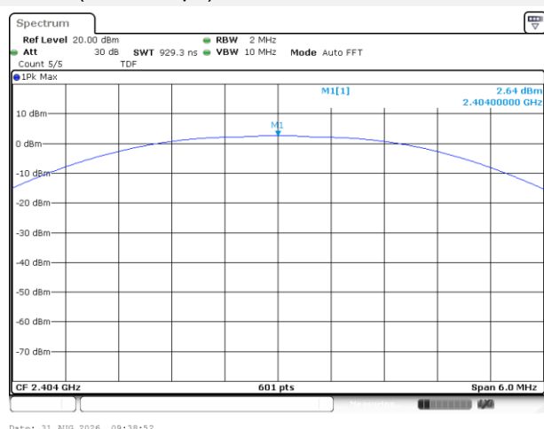
GFSK (BLE 2Mbps) LOW CHANNEL
