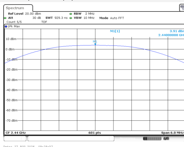
GFSK (BLE 2Mbps) MIDDLE CHANNEL
