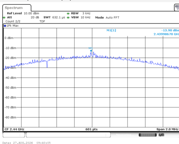
GFSK (BLE 2Mbps) MIDDLE CHANNEL
