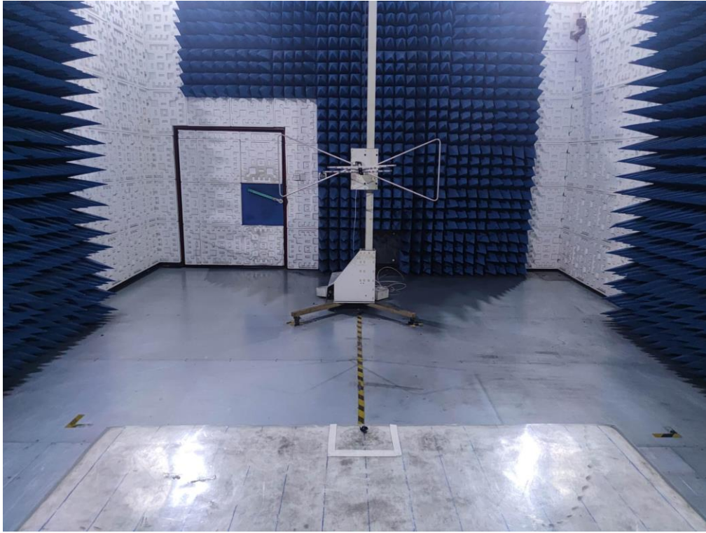
RADIATED EMISSION TEST SETUP BELOW 1GHz- Right earphone
