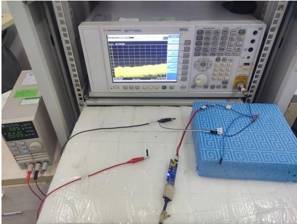
RF CONDUCTED TEST SETUP - Right earphone
