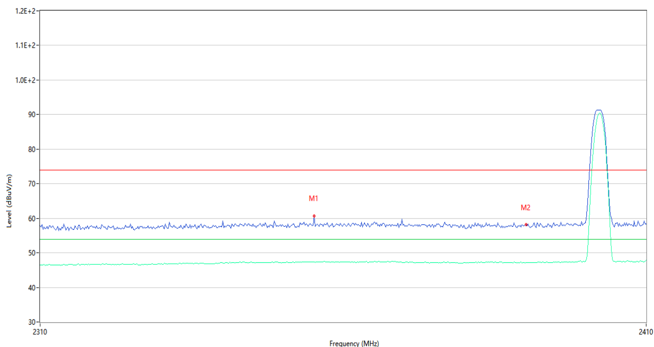
GFSK (BLE 1Mbps) LOW CHANNEL
