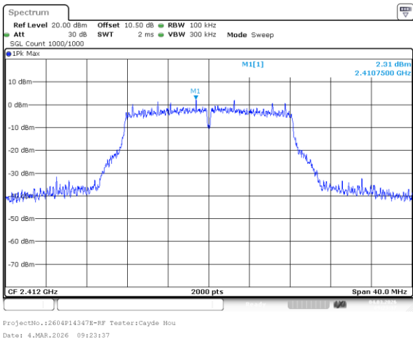
802.11g_2412MHz_Chain 1
