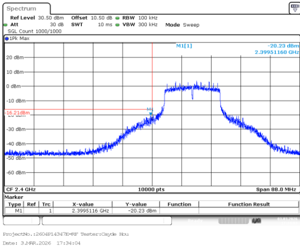
802.11g_2412MHz_Chain 0
