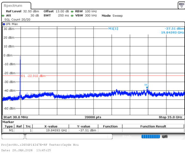
802.11n40_2452MHz_Chain 1
