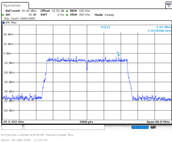
802.11ax40_2422MHz_RU_Full_Chain 0
