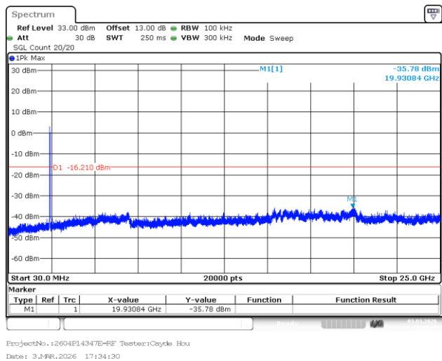
802.11g_2437MHz_Chain 0
