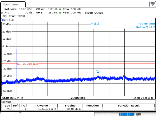
802.11ax40_2422MHz_RU_Full_Chain 1
