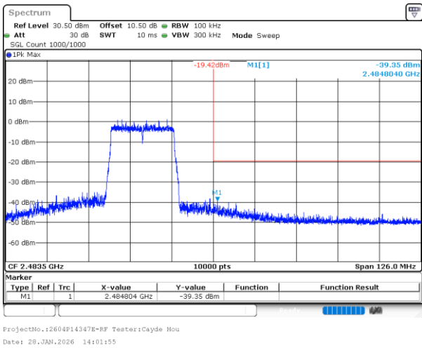
802.11ax20_2462MHz_RU_Full_Chain 1
