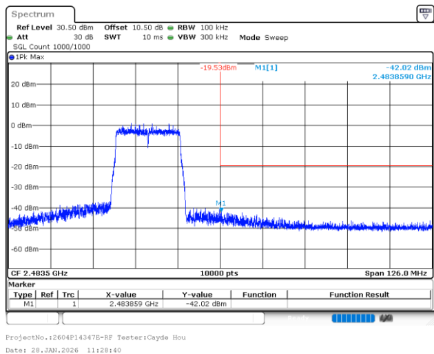
802.11ax20_2462MHz_RU_Full_Chain 0
