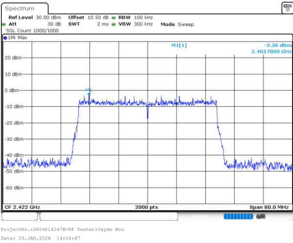
802.11ax40_2422MHz_RU_Full_Chain 1
