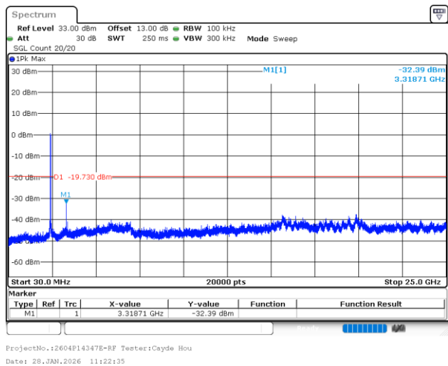
802.11ax20_2437MHz_RU_Full_Chain 0
