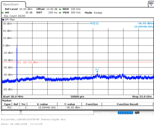
802.11n40_2437MHz_Chain 0
