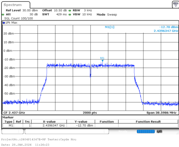
802.11ax20_2437MHz_RU_Full_Chain 0
