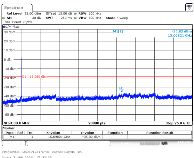
802.11g_2462MHz_Chain 0
