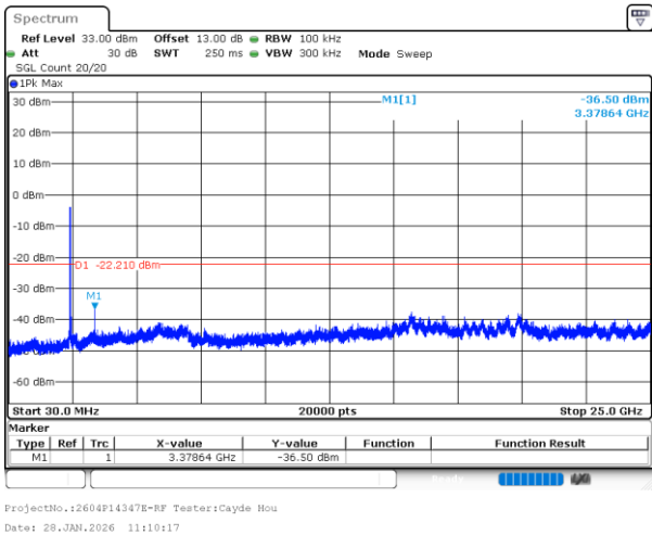
802.11n40_2437MHz_Chain 0
