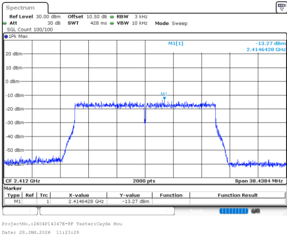
802.11ax20_2412MHz_RU_Full_Chain 0
