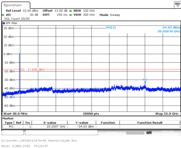
802.11g_2437MHz_Chain 1
