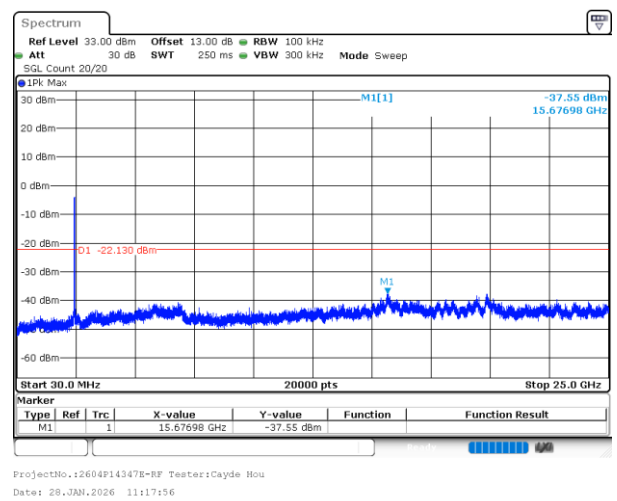
802.11n40_2452MHz_Chain 0
