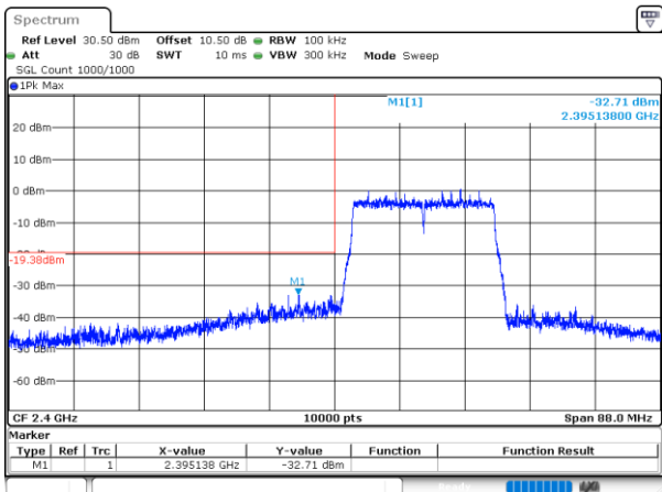
802.11ax20_2412MHz_RU_Full_Chain 1
