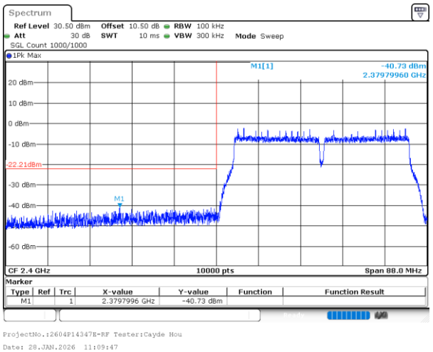
802.11n40_2437MHz_Chain 0
