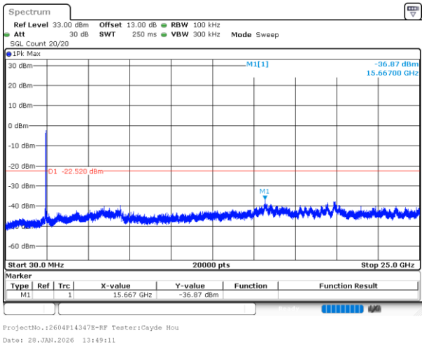
802.11n40_2452MHz_Chain 1
