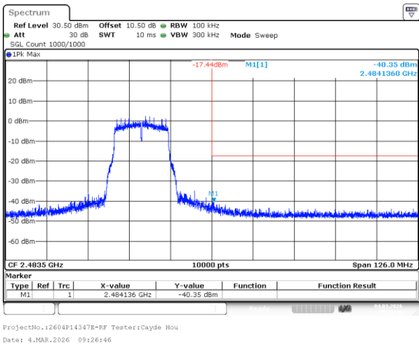
802.11g_2462MHz_Chain 1
