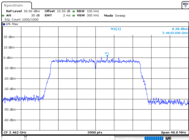
802.11ax20_2462MHz_RU_Full_Chain 1
