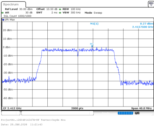
802.11ax20_2412MHz_RU_Full_Chain 0
