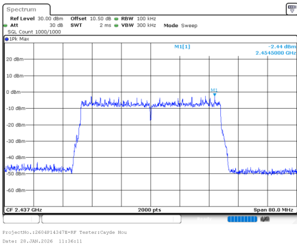
802.11ax40_2437MHz_RU_Full_Chain 0
