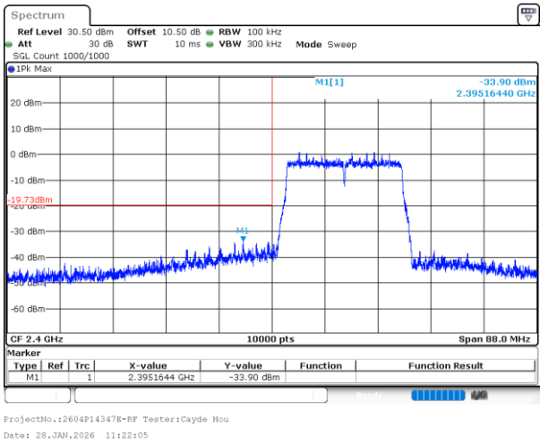
802.11ax20_2412MHz_RU_Full_Chain 0
