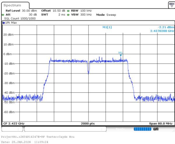
802.11n40_2422MHz_Chain 0
