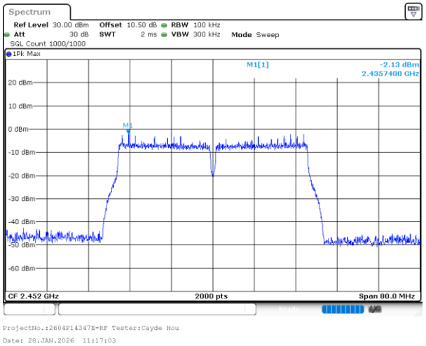
802.11n40_2452MHz_Chain 0
