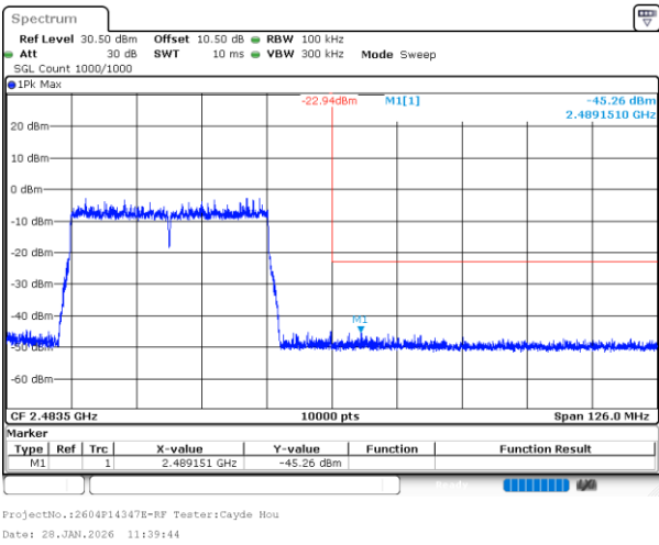
802.11ax40_2452MHz_RU_Full_Chain 0
