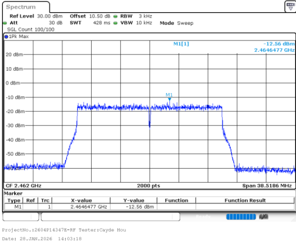
802.11ax20_2462MHz_RU_Full_Chain 1
