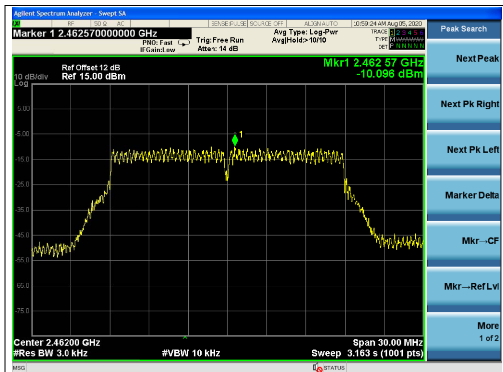
(Channel 11, 802.11n(HT20), ANT L)
