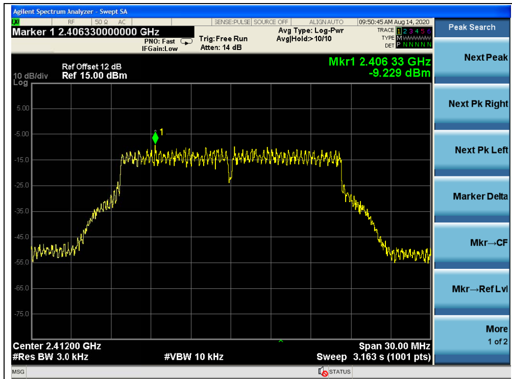
(Channel 1, 802.11g, ANT R)
