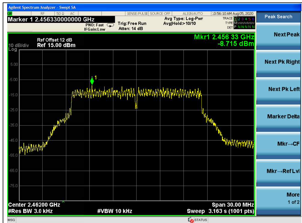
(Channel 11, 802.11g, ANT L)
