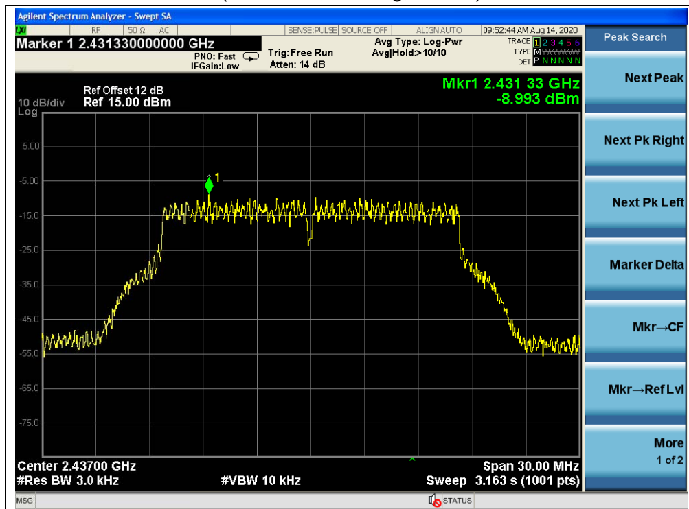
(Channel 6, 802.11g, ANT R)
