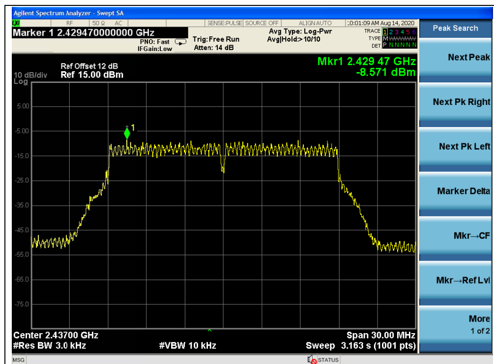
(Channel 6, 802.11n(HT20), ANT R)
