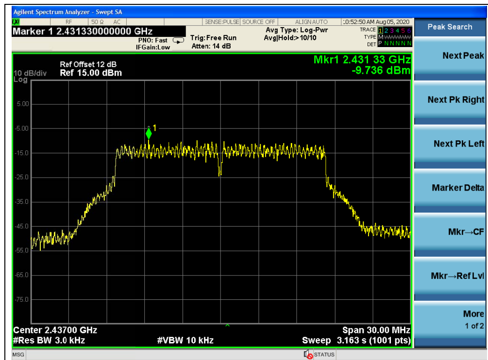
(Channel 6, 802.11g, ANT L)
