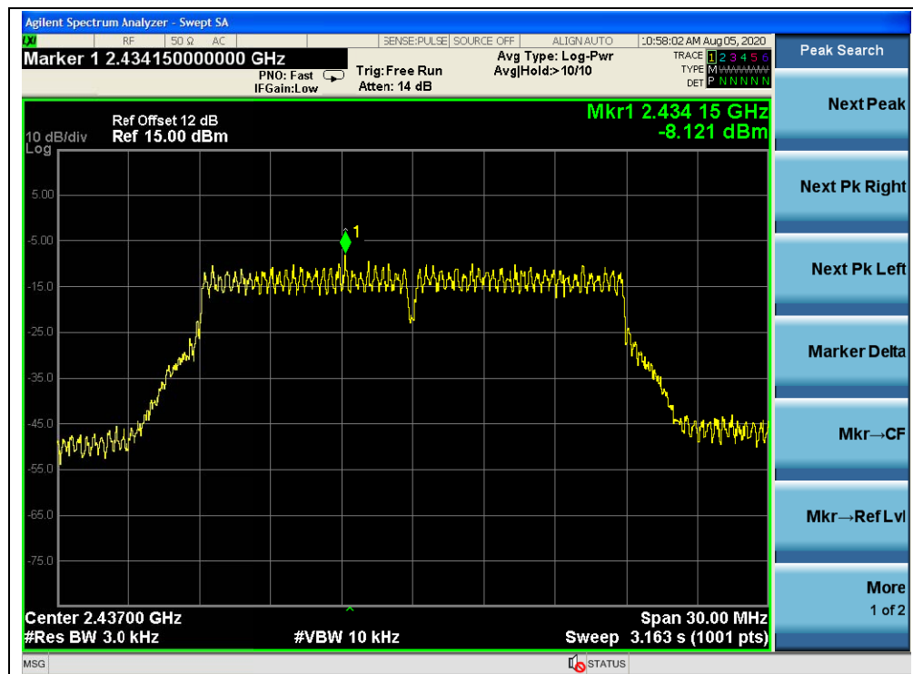
(Channel6, 802.11n(HT20), ANT L)
