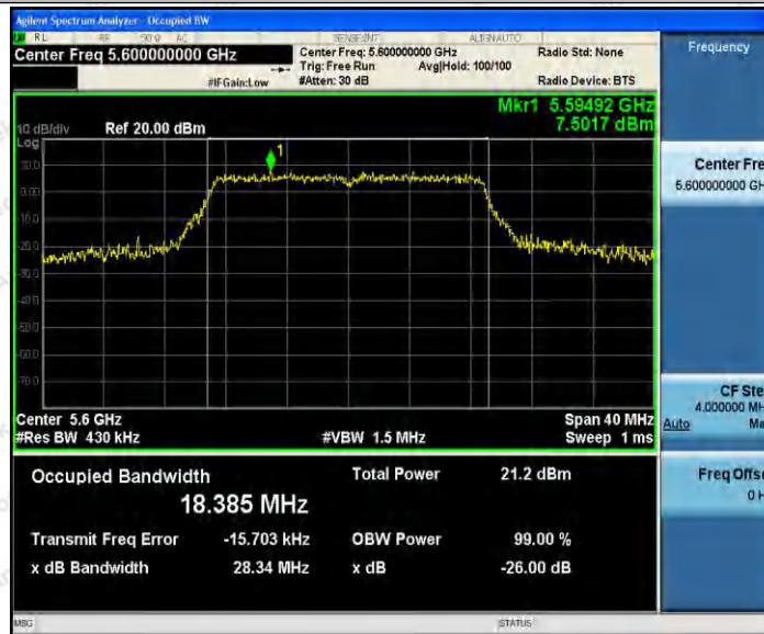
11AC20SISO_Ant2_5600
