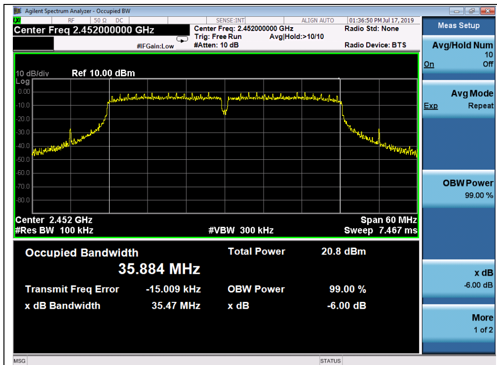
(Channel 9, 802.11n(HT40))
