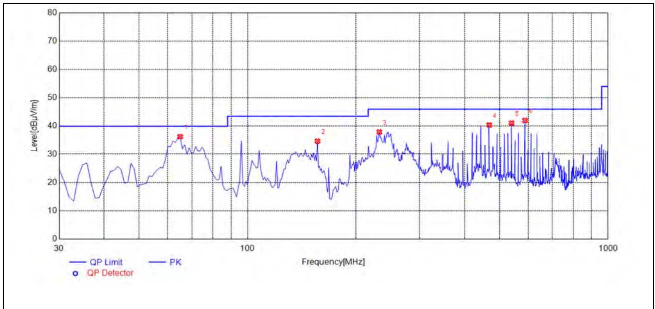
Plot for Channel 78
