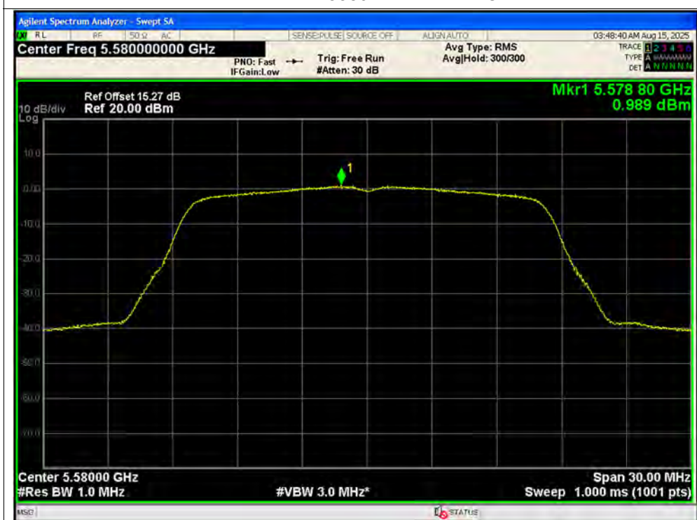
PSD NVNT a 5580MHz Ant2 SISO
