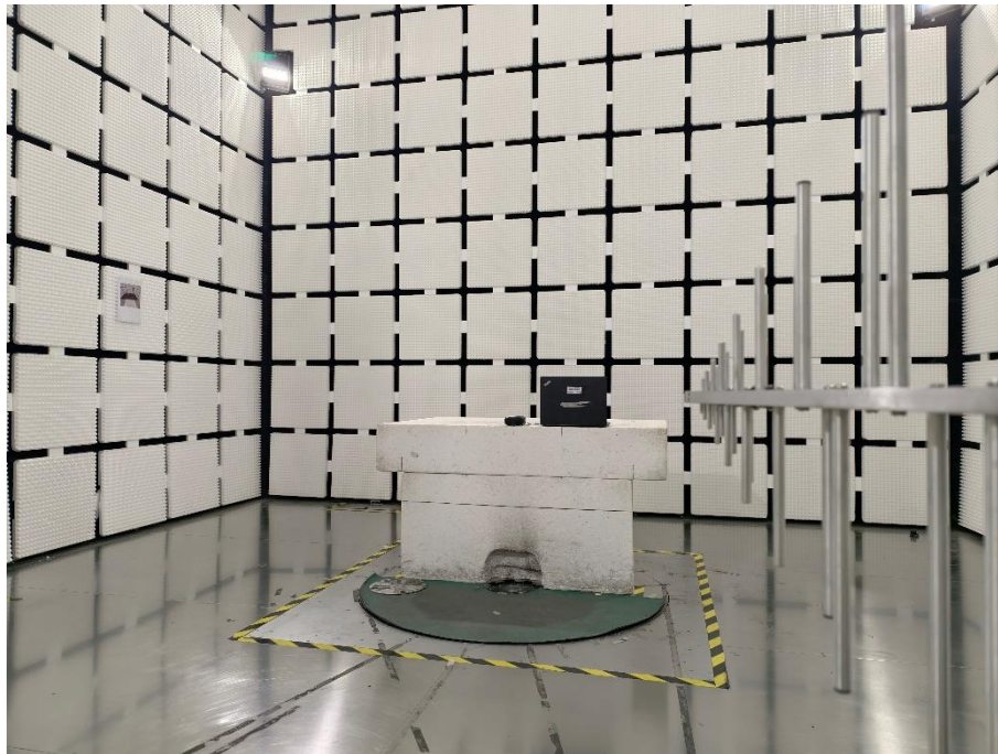
30MHz-1GHz-BT
