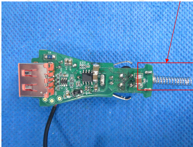
FM Antenna
