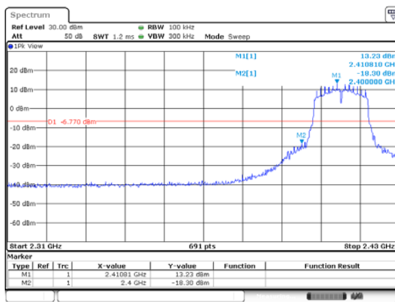
802.11g: Band Edge-Low Channel
