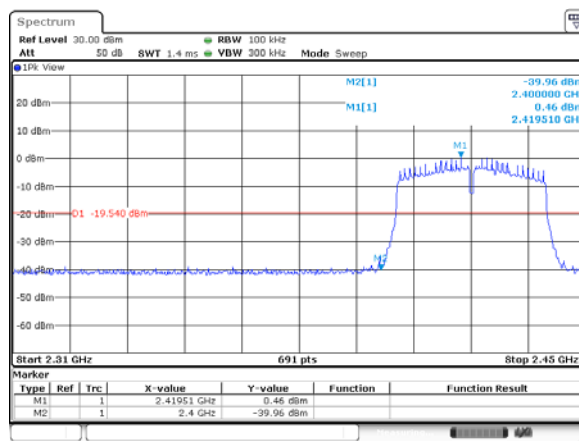
802.11n40: Band Edge-Low Channel
