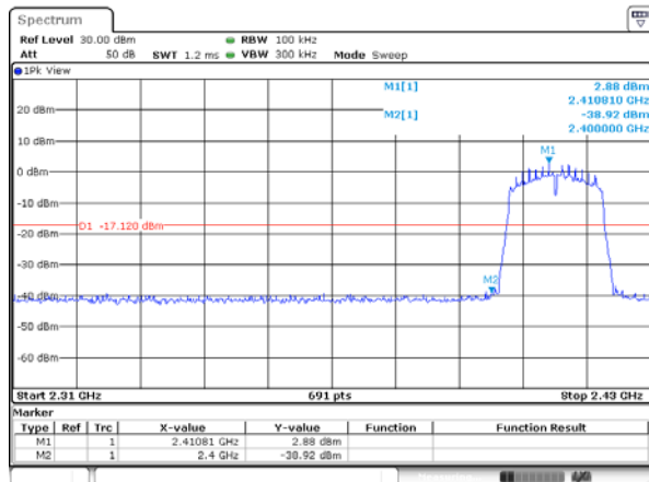
802.11n20: Band Edge-Low Channel
