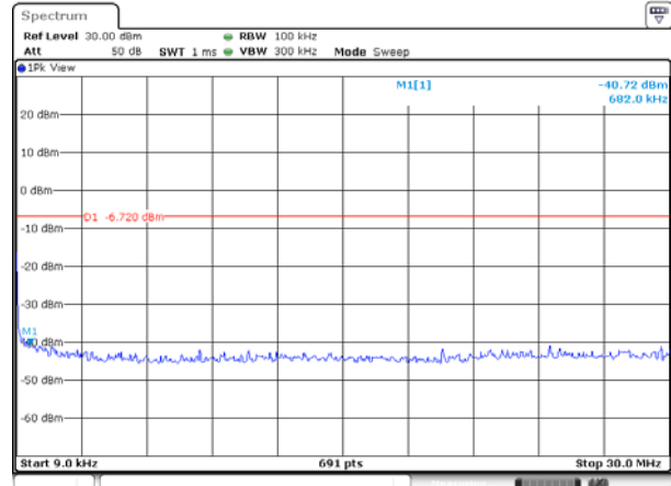
GFSK on channel 05
