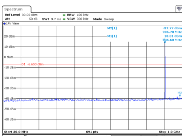
GFSK on channel 03
