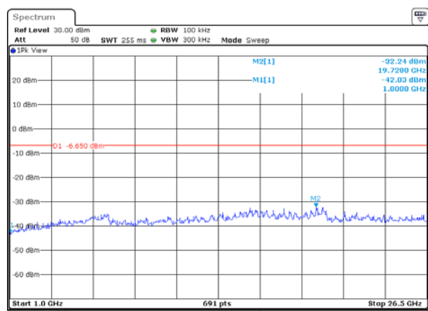
GFSK on channel 03
