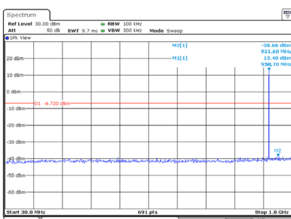
GFSK on channel 05
