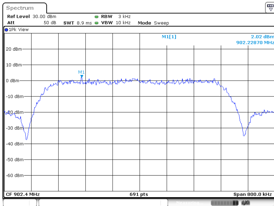
Power spectral density plot on channel 01
