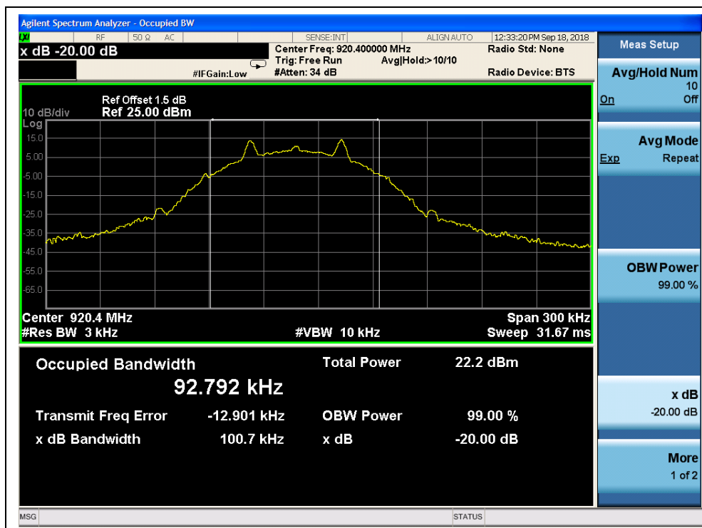
(Channel 3, 920.4 MHz)
