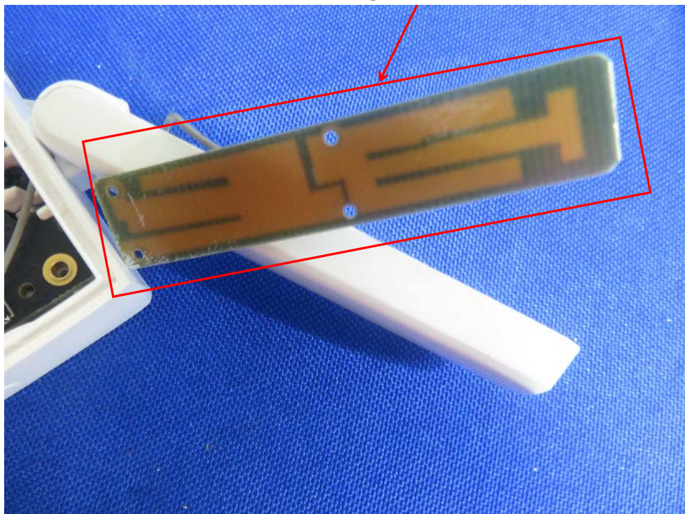
2.4G WiFi ANT B
