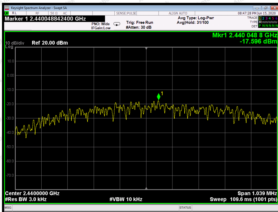
CH: 1M-Middle
