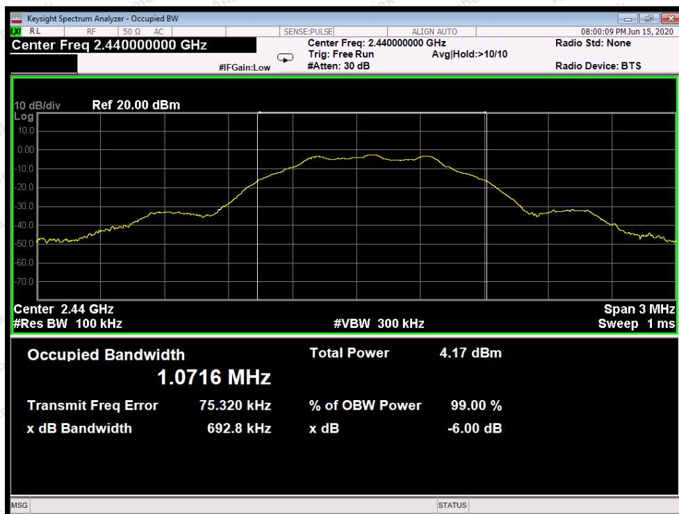
CH: 1M-Middle
