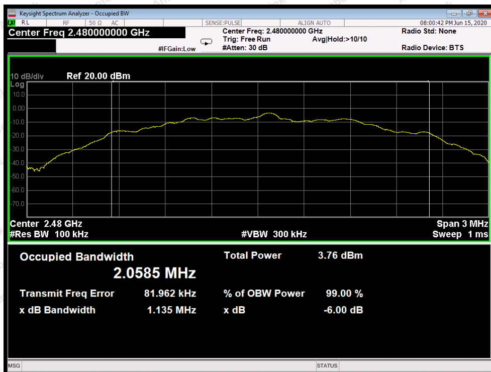
CH: 2M-High
