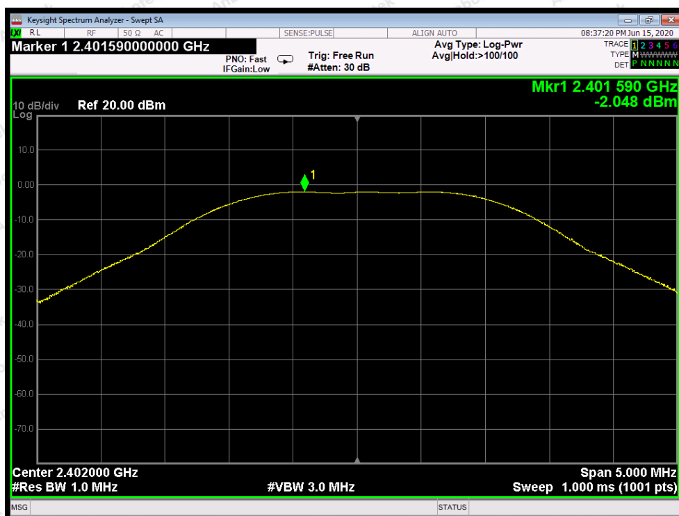
CH: 2M-Low
