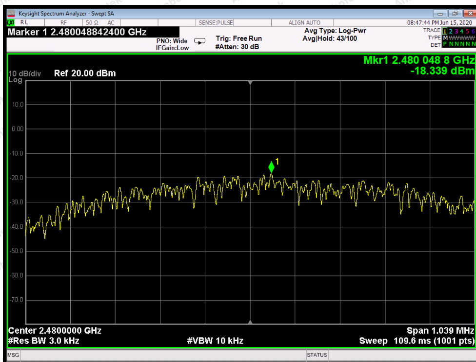
CH: 1M-High
