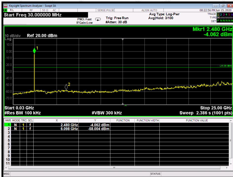
CH: 2M-High
