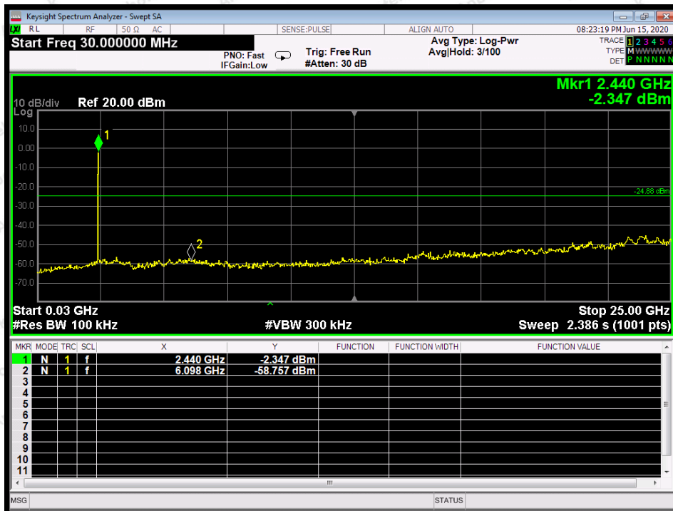
CH: 2M-Middle
