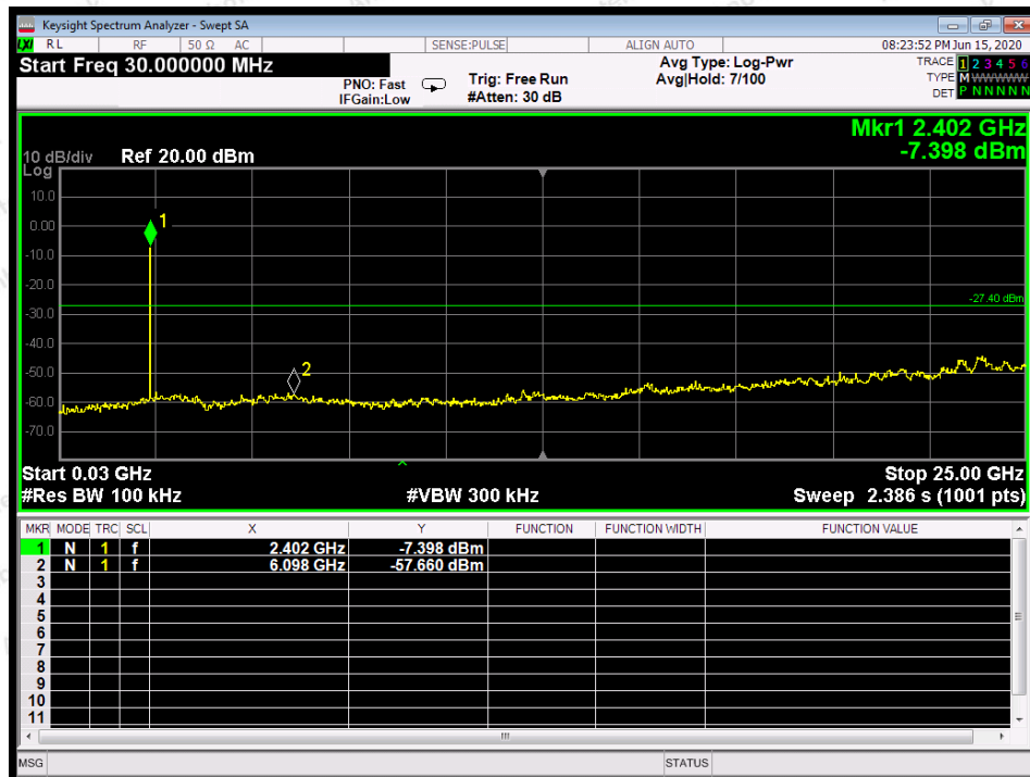
CH: 2M-Low
