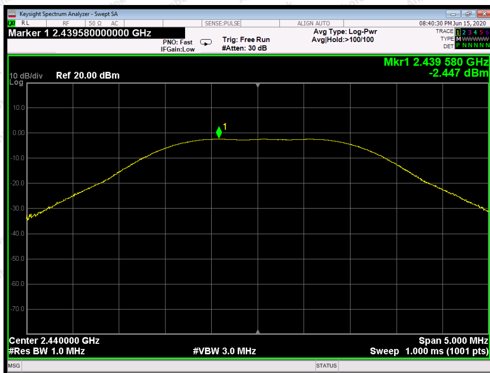
CH: 2M-Middle
