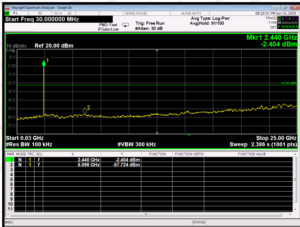
CH: 1M-Middle
