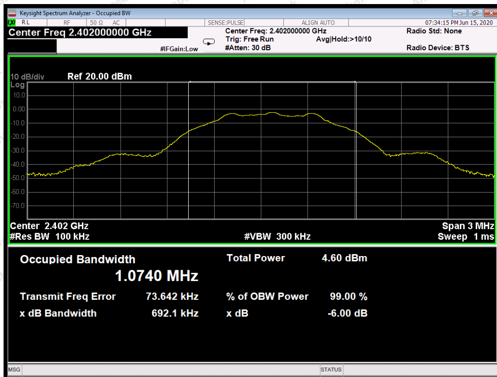
CH: 1M-Low
