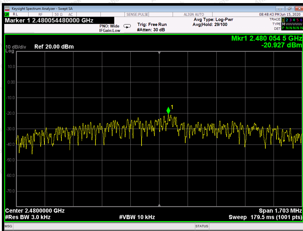
CH: 2M-High
