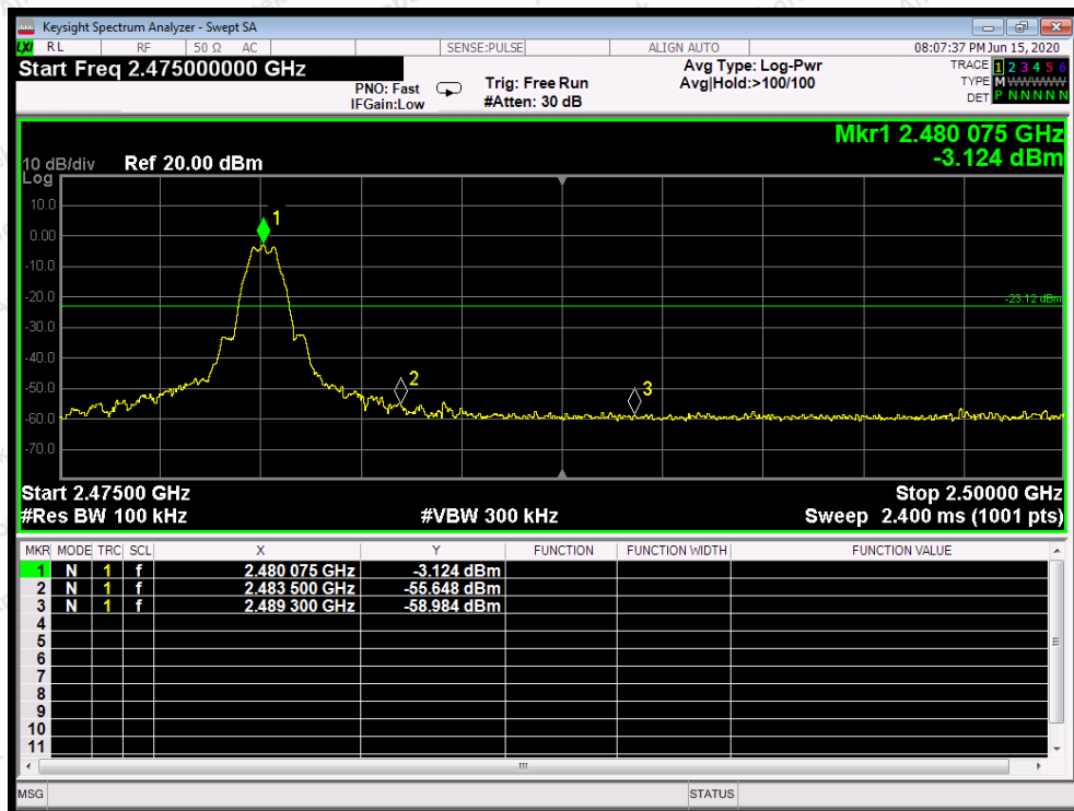
CH: 1M-High
