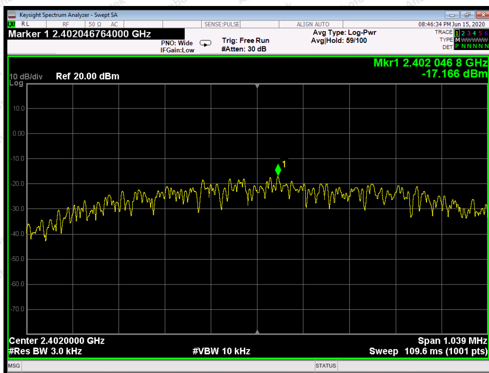
CH: 1M-Low
