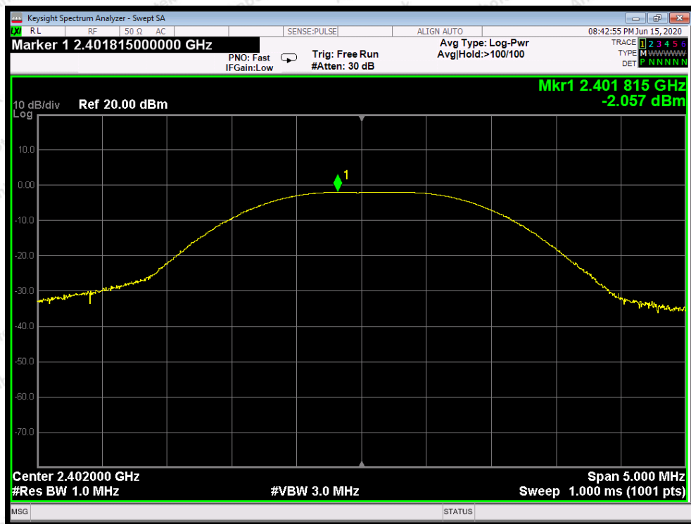
CH: 1M-Low
