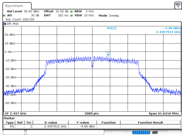
802.11g_2437MHz_Chain 1
