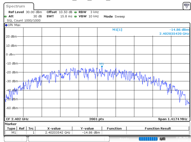
BLE_1M_Low_Channel
