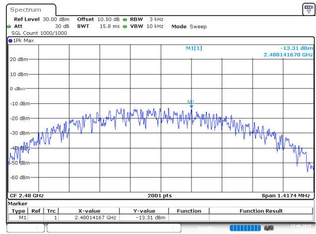
BLE_1M_High_Channel
