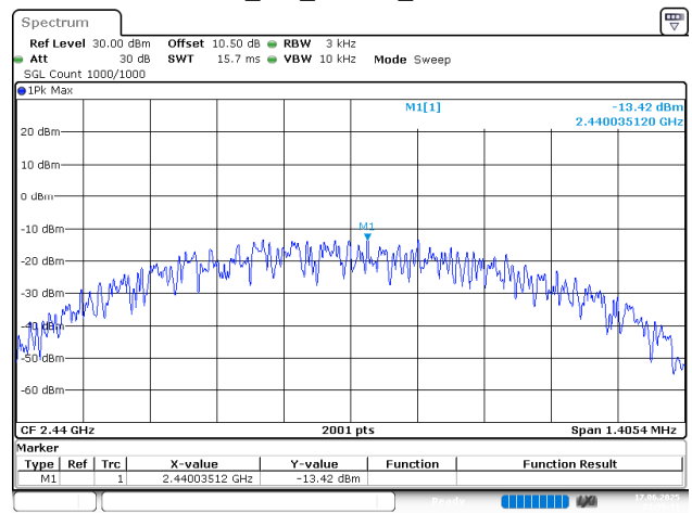
BLE_1M_Middle_Channel
