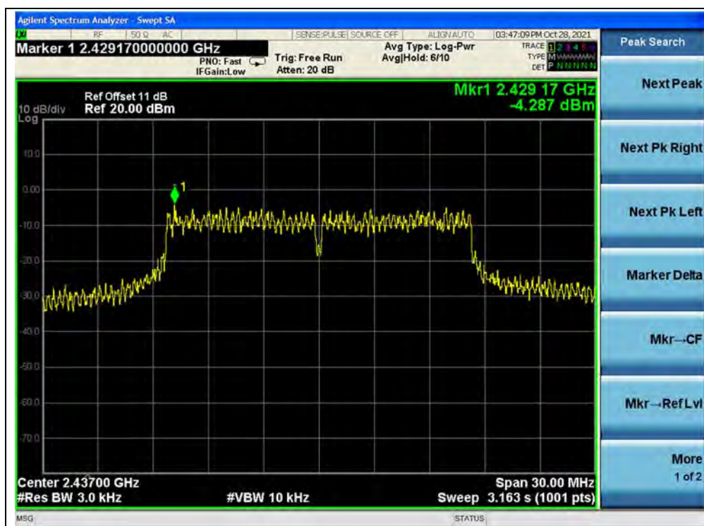
(Channel 6, 802.11g)
