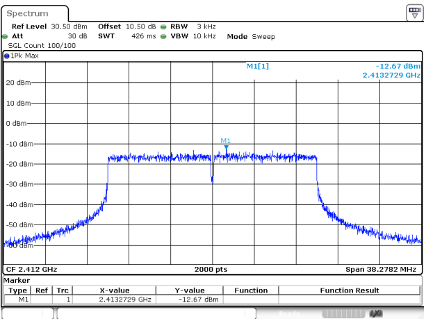
802.11ax20_2412MHz_RU_Full
