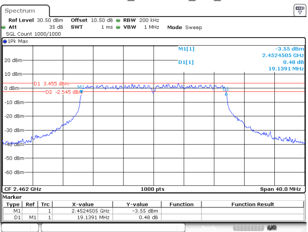
802.11ax20_2462MHz_RU_Full
