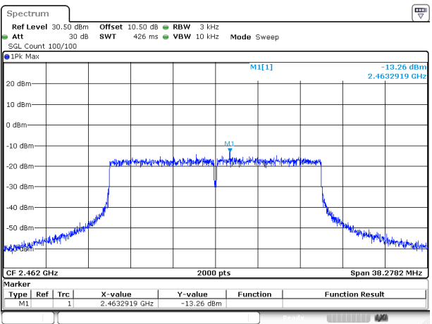
802.11ax20_2462MHz_RU_Full
