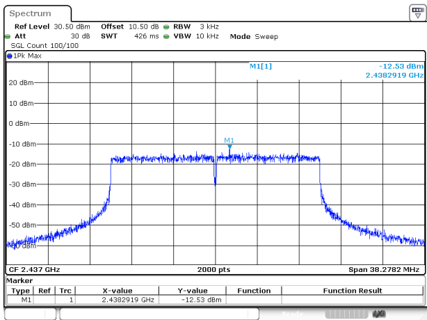
802.11ax20_2437MHz_RU_Full
