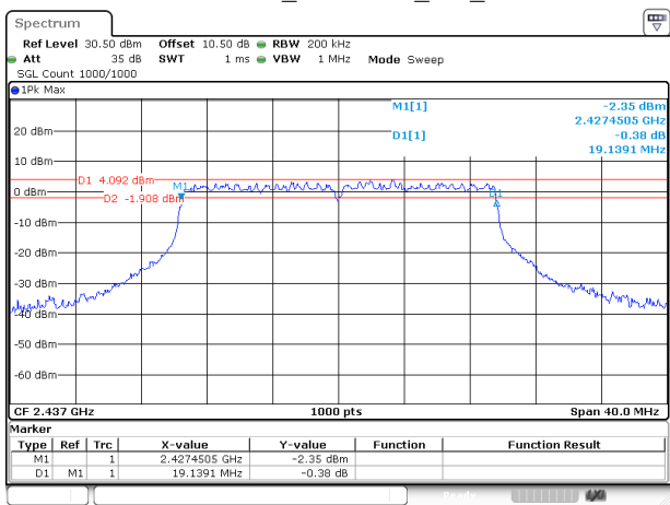
802.11ax20_2437MHz_RU_Full
