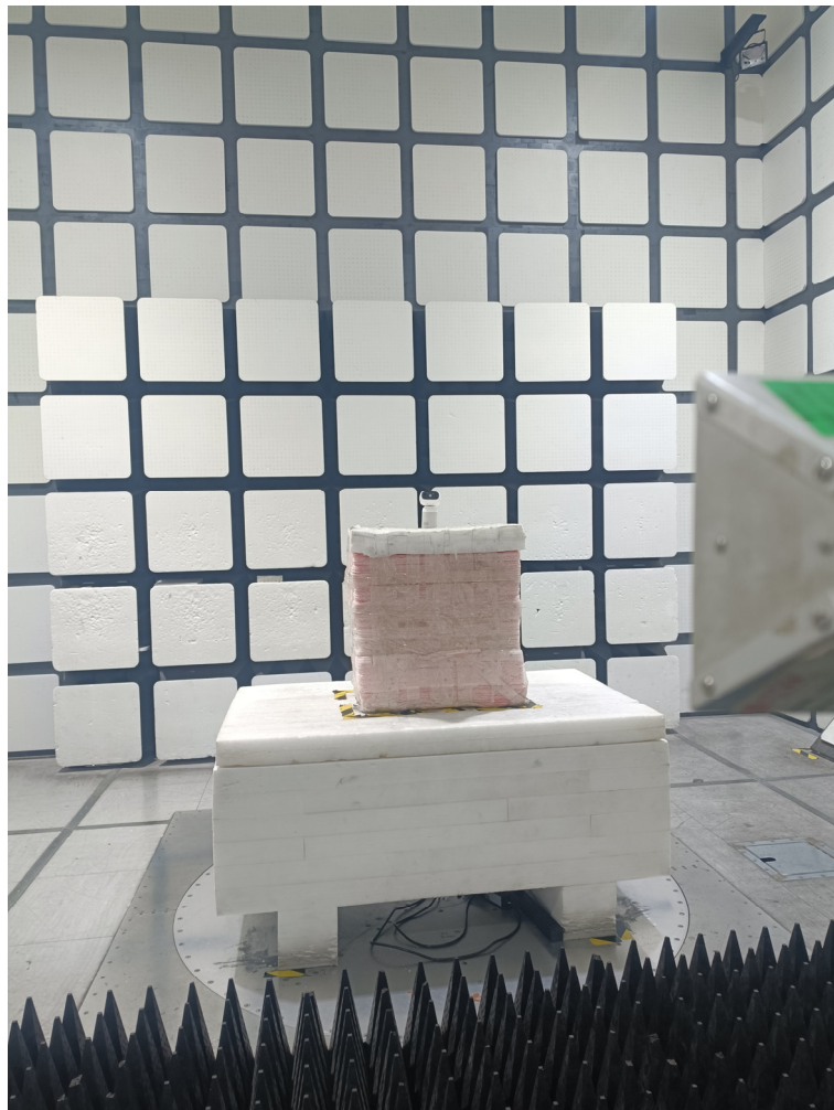
Radiated Emissions View (18-25 GHz)
