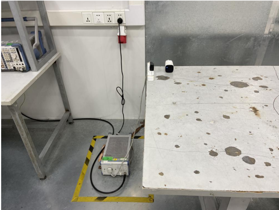
FCC ID: 2AOKB-T8130X Photo of Power Line Conducted Emission Test
