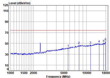
11g_TX_CH_11_Vertical-Peak
