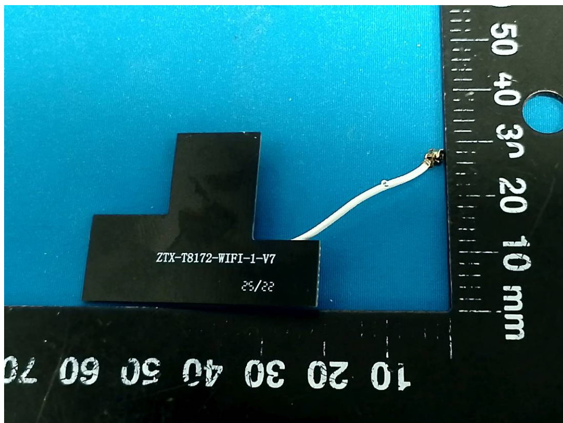
BLE&Wifi Antenna(Chain 1)
