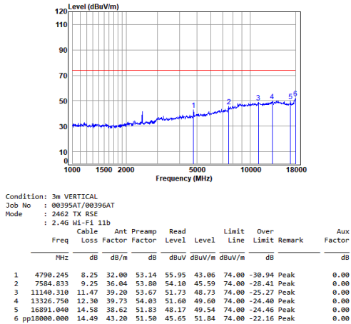
11b_TX_CH_11_Vertical-Peak
