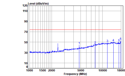
11b_TX_CH_06_Vertical-Peak
