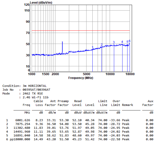
11b_TX_CH_11_Horizontal-Peak
