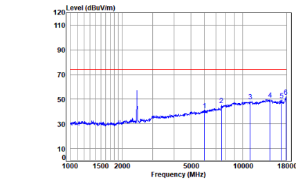
11b_TX_CH_06_Horizontal-Peak
