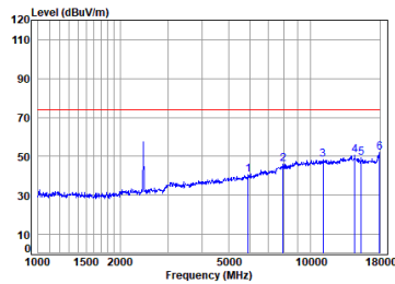
11n_20M_TX_CH_06_Horizontal-Peak
