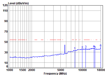
11ax_20M_TX_CH_149_Vertical-Avg
