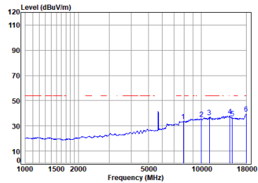
11ax_20M_TX_CH_140_Horizontal-Avg
