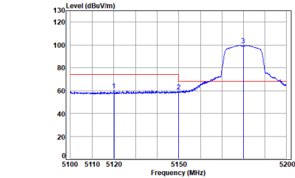
11ac_VHT(20M)_TX_CH_36_Horizontal-Peak
