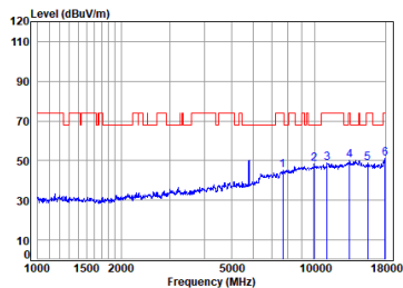
11ax_20M_TX_CH_157_Horizontal-Peak
