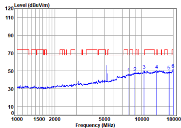
11ax_20M_TX_CH_52_Horizontal-Peak
