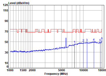
11a_TX_CH_157_Horizontal-Peak
