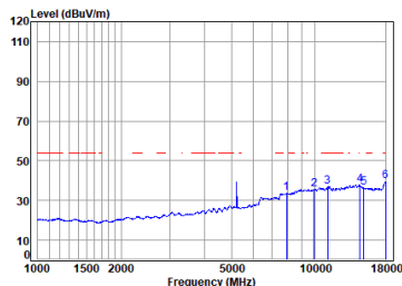
11ax_20M_TX_CH_44_Horizontal-Avg
