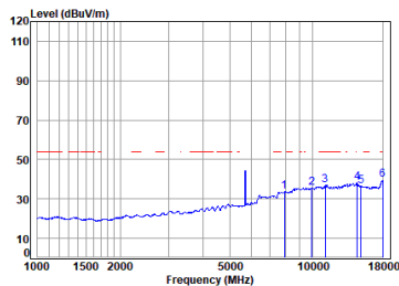
11a_TX_CH_140_Horizontal-Avg
