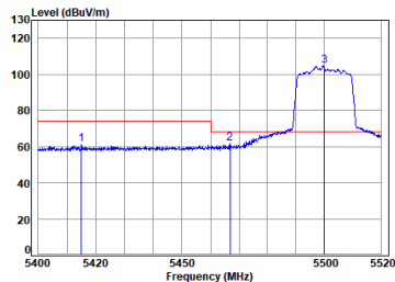
11ac_VHT(20M)_TX_CH_100_Horizontal-Peak
