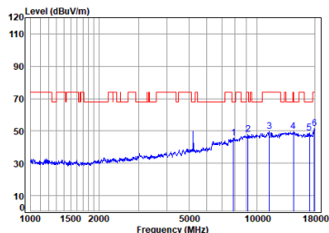
11ax_20M_TX_CH_44_Horizontal-Peak
