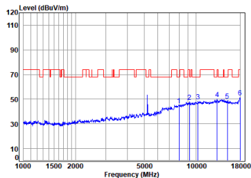
11ax_20M_TX_CH_44_Vertical-Peak
