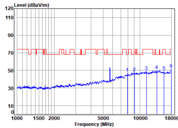
11ax_20M_TX_CH_140_Horizontal-Peak
