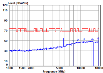
11ax_20M_TX_CH_157_Vertical-Peak
