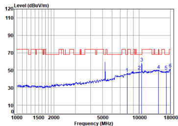
11ax_20M_TX_CH_52_Vertical-Peak
