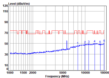
11a_TX_CH_140_Horizontal-Peak
