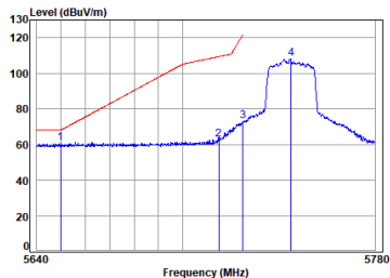
11ax_20M_TX_CH_149_Vertical
