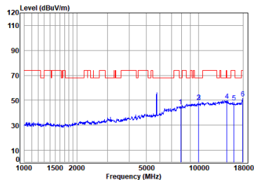
11ax_20M_TX_CH_149_Vertical-Peak
