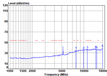
11ax_20M_TX_CH_44_Vertical-Avg
