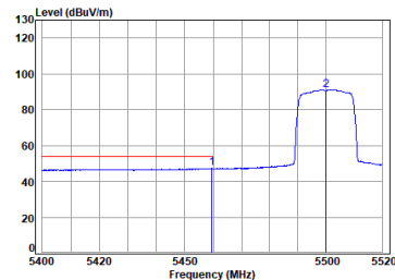
11ac_VHT(20M)_TX_CH_100_Horizontal-Avg
