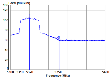
11ax_20M_TX_CH_64_Horizontal-Peak
