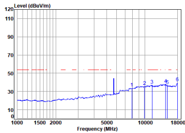
11a_TX_CH_140_Vertical-Avg
