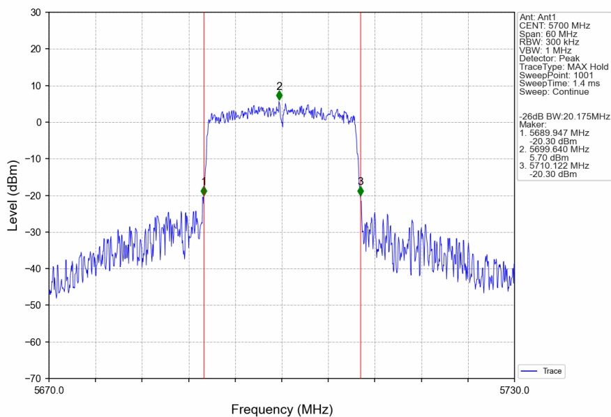
802.11ax(HEW20)_HCH_5700MHz_SU_/_Ant1_NTNV
