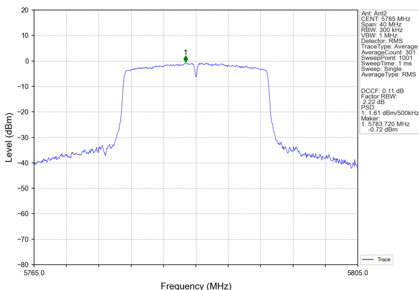
802.11n(HT20)_MCH_5785MHz_Ant2_NTNV
