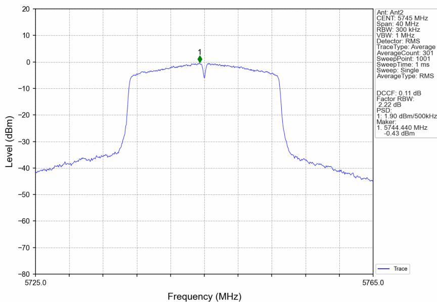
802.11ac(VHT20)_LCH_5745MHz_Ant2_NTNV
