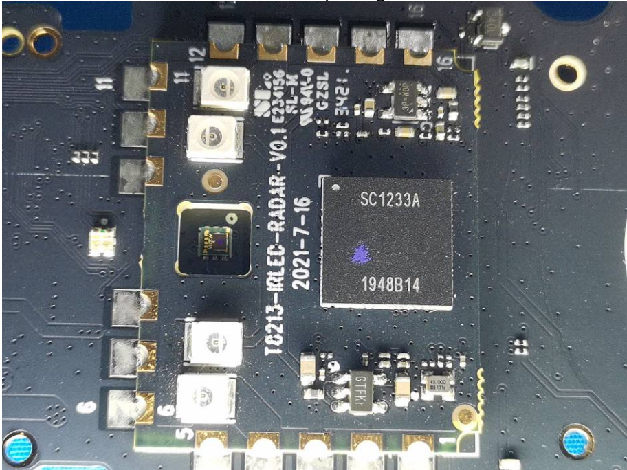
24G Chip Integrated Antenna
