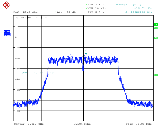
802.11g_2412MHz
