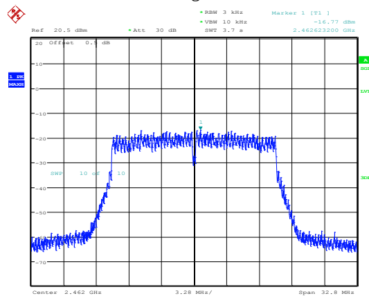
802.11g_2462MHz
