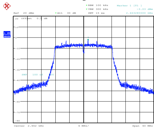
802.11g_2462MHz
