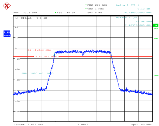
802.11g_2412MHz
