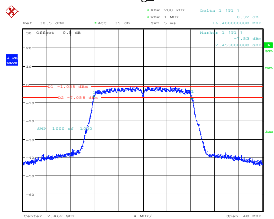
802.11g_2462MHz
