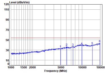
Antenna 1 BLE_1M_TX_CH_39_Horizontal-Avg
