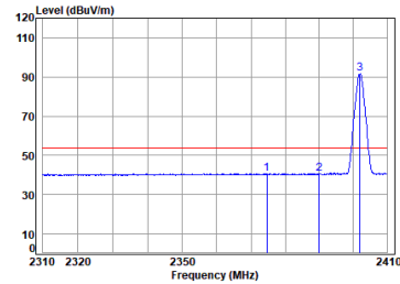
Antenna 0 BLE_2M_TX_CH_00_Vertical-Avg
