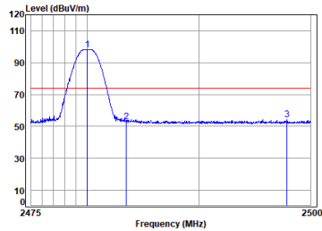
Antenna 1 BLE_1M_TX_CH_39_Vertical-Peak
