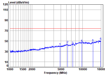
Antenna 0 BLE_2M_TX_CH_19_Horizontal-Peak
