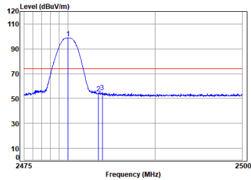
Antenna 0 BLE_1M_TX_CH_39_Vertical-Peak
