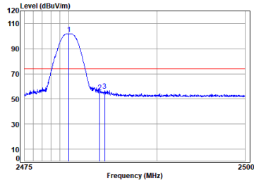
Antenna 0 BLE_1M_TX_CH_39_Horizontal-Peak
