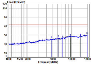
Antenna 0 BLE_2M_TX_CH_00_Horizontal-Peak
