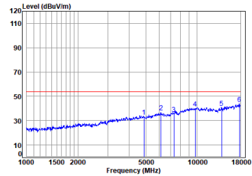
Antenna 1 BLE_1M_TX_CH_19_Vertical-Avg
