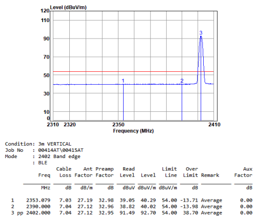
Antenna 0 BLE_1M_TX_CH_00_Vertical-Avg
