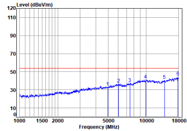
Antenna 0 BLE_1M_TX_CH_39_Vertical-Avg
