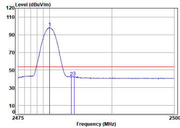
Antenna 0 BLE_1M_TX_CH_39_Vertical-Avg
