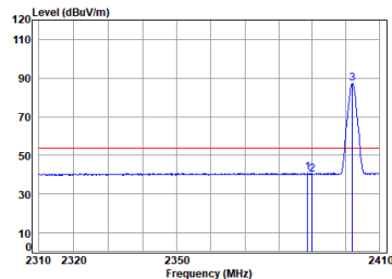
Antenna 1 BLE_2M_TX_CH_00_Vertical-Avg
