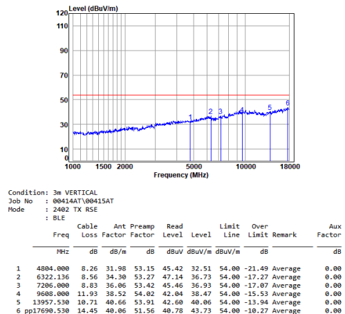
Antenna 0 BLE_1M_TX_CH_00_Vertical-Avg
