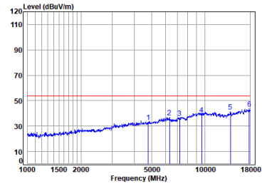
Antenna 1 BLE_2M_TX_CH_00_Vertical-Avg
