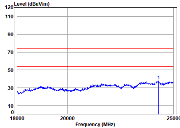
Antenna 0 BLE_1M_TX_CH_19_Horizontal-Peak
