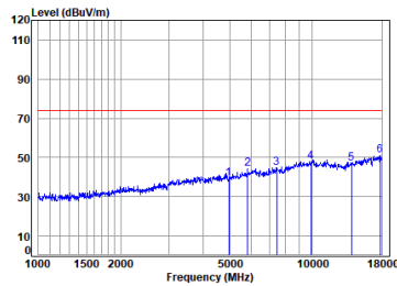
Antenna 0 BLE_2M_TX_CH_39_Vertical-Peak
