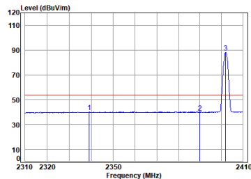
Antenna 1 BLE_1M_TX_CH_00_Vertical-Avg
