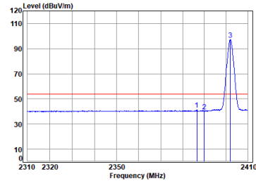
Antenna 0 BLE_2M_TX_CH_00_Horizontal-Avg
