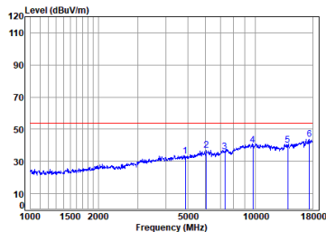
Antenna 0 BLE_1M_TX_CH_19_Vertical-Avg
