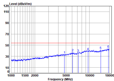
Antenna 1 BLE_1M_TX_CH_00_Horizontal-Avg
