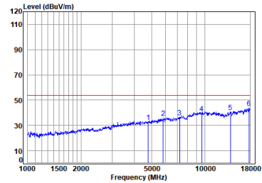
Antenna 0 BLE_2M_TX_CH_00_Vertical-Avg
