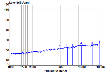
Antenna 1 BLE_2M_TX_CH_19_Vertical-Avg
