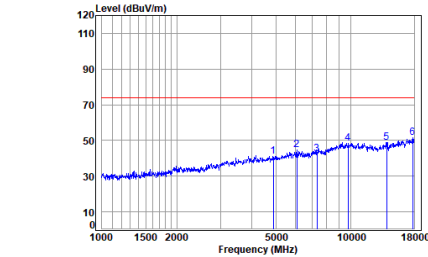
Antenna 1 BLE_2M_TX_CH_19_Horizontal-Peak
