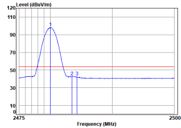
Antenna 1 BLE_1M_TX_CH_39_Vertical-Avg
