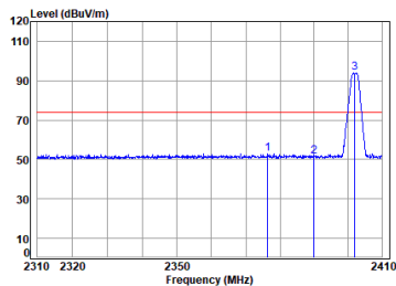
Antenna 1 BLE_2M_TX_CH_00_Horizontal-Peak
