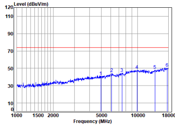
Antenna 0 BLE_2M_TX_CH_39_Horizontal-Peak
