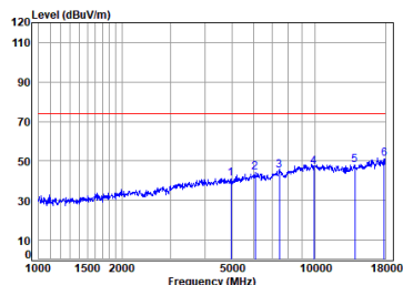
Antenna 1 BLE_2M_TX_CH_39_Vertical-Peak
