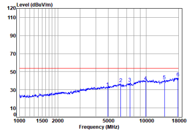
Antenna 1 BLE_1M_TX_CH_39_Vertical-Avg
