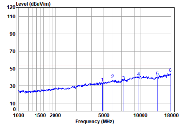
Antenna 0 BLE_2M_TX_CH_19_Horizontal-Avg
