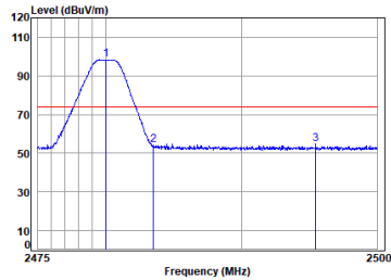
Antenna 1 BLE_2M_TX_CH_39_Vertical-Peak
