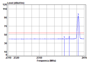
Antenna 1 BLE_1M_TX_CH_00_Horizontal-Avg
