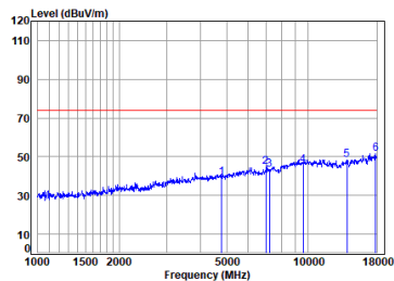
Antenna 1 BLE_1M_TX_CH_00_Horizontal-Peak
