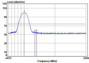
Antenna 1 BLE_1M_TX_CH_39_Horizontal-Peak
