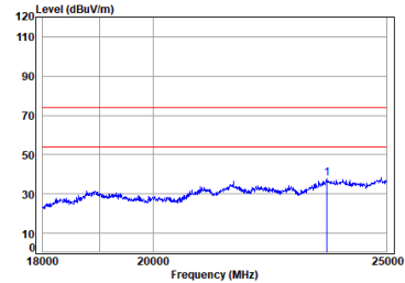
Antenna 0 BLE_1M_TX_CH_19_Vertical-Peak
