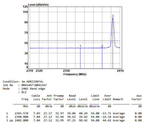
Antenna 0 BLE_1M_TX_CH_00_Horizontal-Avg
