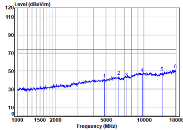
Antenna 1 BLE_1M_TX_CH_19_Horizontal-Peak
