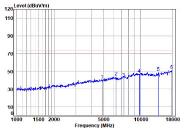
Antenna 0 BLE_1M_TX_CH_19_Vertical-Peak
