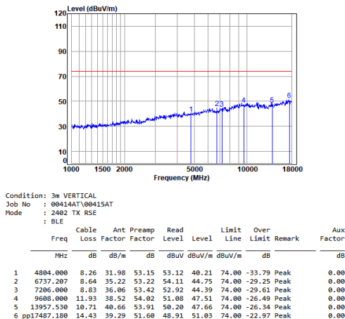
Antenna 0 BLE_1M_TX_CH_00_Vertical-Peak
