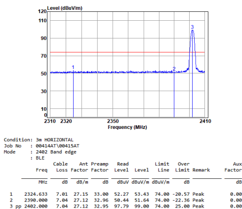
Antenna 0 BLE_1M_TX_CH_00_Horizontal-Peak
