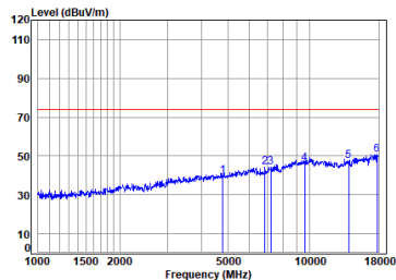
Antenna 1 BLE_1M_TX_CH_00_Vertical-Peak
