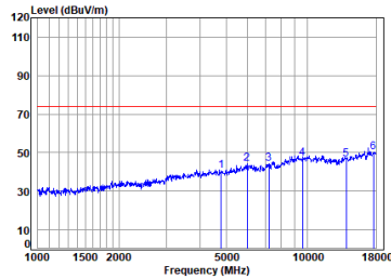
Antenna 0 BLE_2M_TX_CH_00_Vertical-Peak
