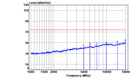
Antenna 0 BLE_1M_TX_CH_39_Vertical-Peak
