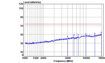
Antenna 1 BLE_1M_TX_CH_39_Vertical-Peak
