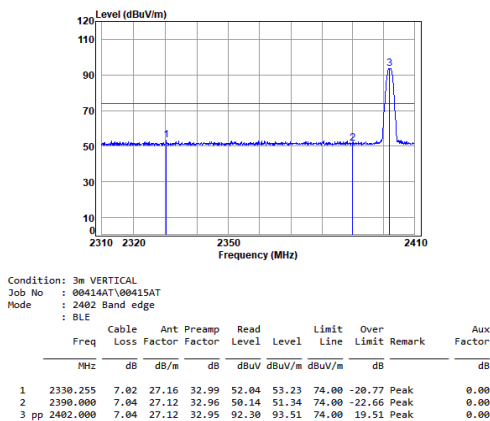
Antenna 0 BLE_1M_TX_CH_00_Vertical-Peak
