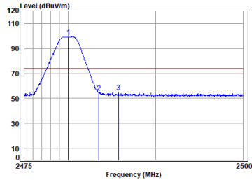
Antenna 1 BLE_2M_TX_CH_39_Horizontal-Peak
