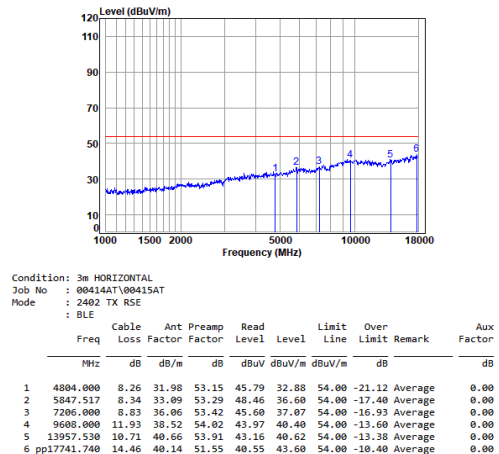
Antenna 0 BLE_1M_TX_CH_00_Horizontal-Avg
