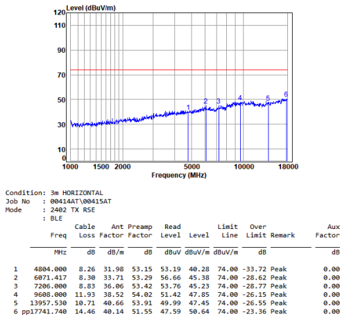
Antenna 0 BLE_1M_TX_CH_00_Horizontal-Peak
