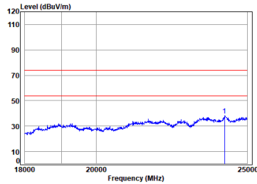
Antenna 1 BLE_1M_TX_CH_19_Horizontal-Peak
