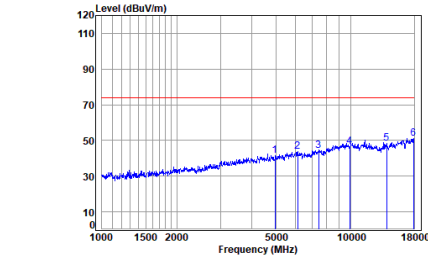
Antenna 1 BLE_1M_TX_CH_39_Horizontal-Peak
