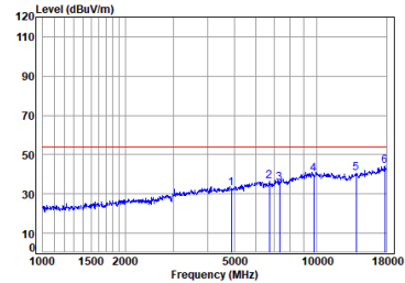
Antenna 1 BLE_2M_TX_CH_19_Horizontal-Avg
