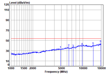
Antenna 0 BLE_2M_TX_CH_19_Vertical-Avg
