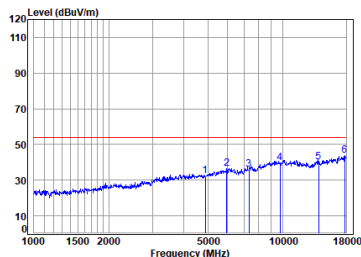
Antenna 0 BLE_1M_TX_CH_19_Horizontal-Avg
