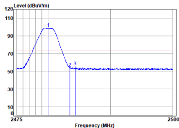
Antenna 0 BLE_2M_TX_CH_39_Vertical-Peak
