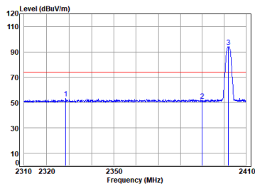
Antenna 1 BLE_1M_TX_CH_00_Horizontal-Peak
