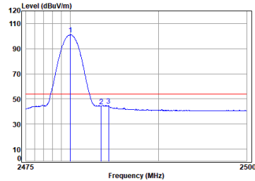
Antenna 0 BLE_1M_TX_CH_39_Horizontal-Avg
