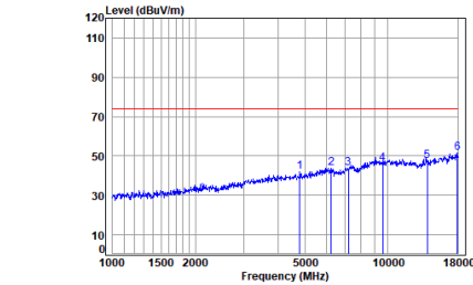
Antenna 1 BLE_2M_TX_CH_00_Vertical-Peak
