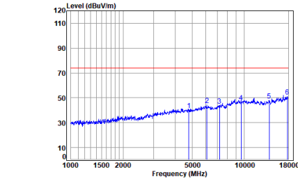
Antenna 1 BLE_2M_TX_CH_00_Horizontal-Peak
