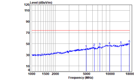
Antenna 0 BLE_1M_TX_CH_39_Horizontal-Peak
