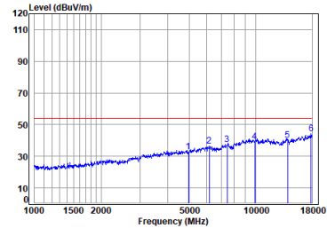
Antenna 0 BLE_1M_TX_CH_39_Horizontal-Avg
