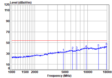
Antenna 0 BLE_2M_TX_CH_00_Horizontal-Avg
