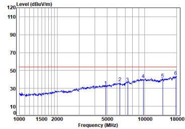
Antenna 1 BLE_1M_TX_CH_19_Horizontal-Avg
