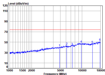
Antenna 0 BLE_1M_TX_CH_19_Horizontal-Peak
