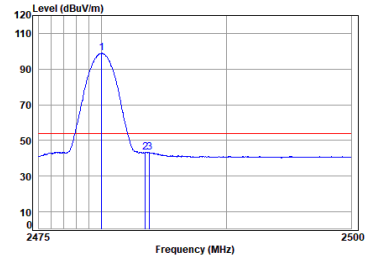
Antenna 1 BLE_1M_TX_CH_39_Horizontal-Avg
