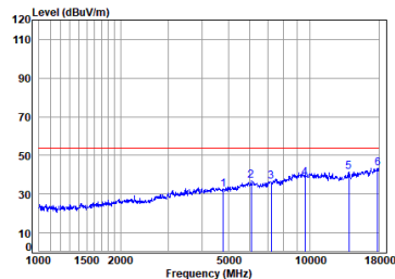
Antenna 1 BLE_1M_TX_CH_00_Vertical-Avg
