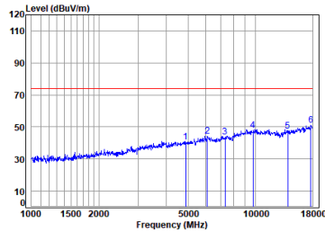
Antenna 1 BLE_1M_TX_CH_19_Vertical-Peak
