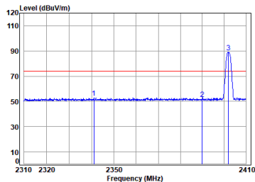
Antenna 1 BLE_1M_TX_CH_00_Vertical-Peak
