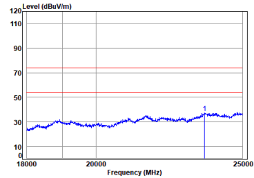
Antenna 1 BLE_1M_TX_CH_19_Vertical-Peak
