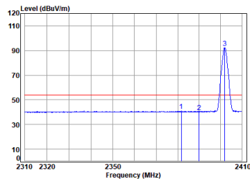
Antenna 1 BLE_2M_TX_CH_00_Horizontal-Avg
