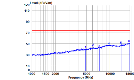
Antenna 1 BLE_2M_TX_CH_19_Vertical-Peak
