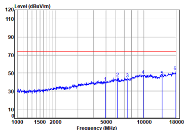
Antenna 1 BLE_2M_TX_CH_39_Horizontal-Peak
