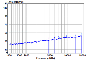
Antenna 1 BLE_2M_TX_CH_00_Horizontal-Avg
