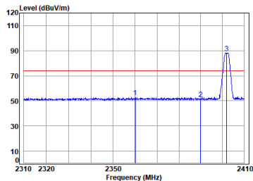
Antenna 1 BLE_2M_TX_CH_00_Vertical-Peak
