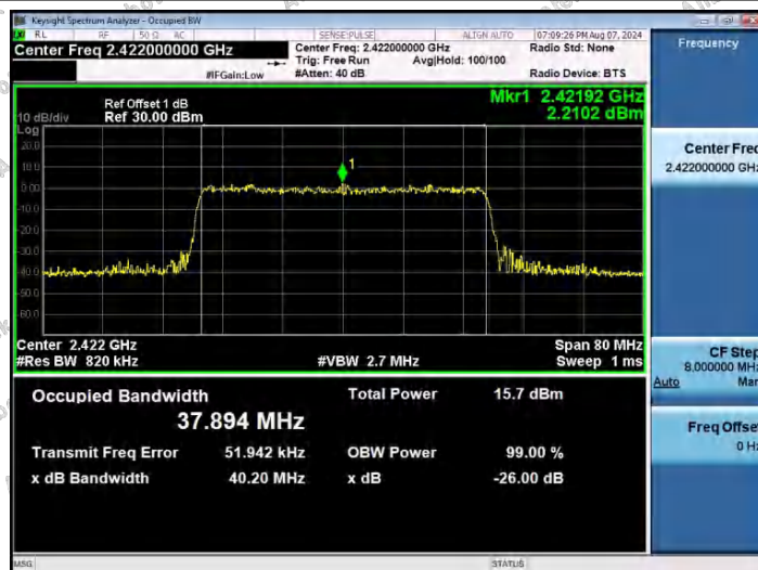
11AX40SISO-Ant1-2422
