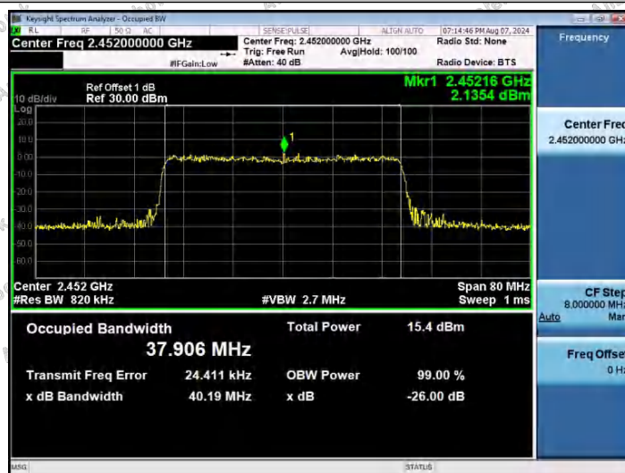
11AX40SISO-Ant1-2452
