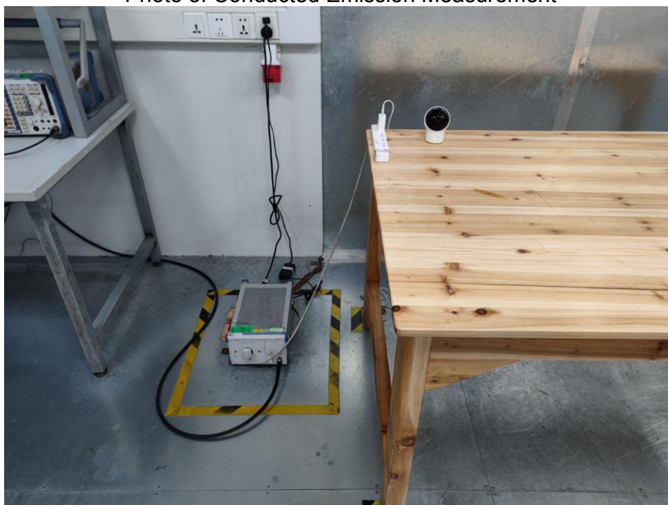
FCC ID: 2AOKB-T8360 Photo of Conducted Emission Measurement
